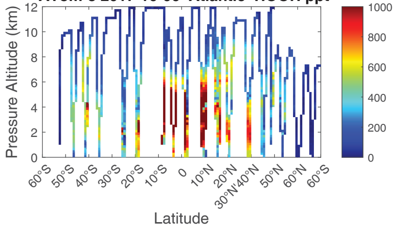
ATom-3 2017-10-06 Atlantic HOOH ppt
