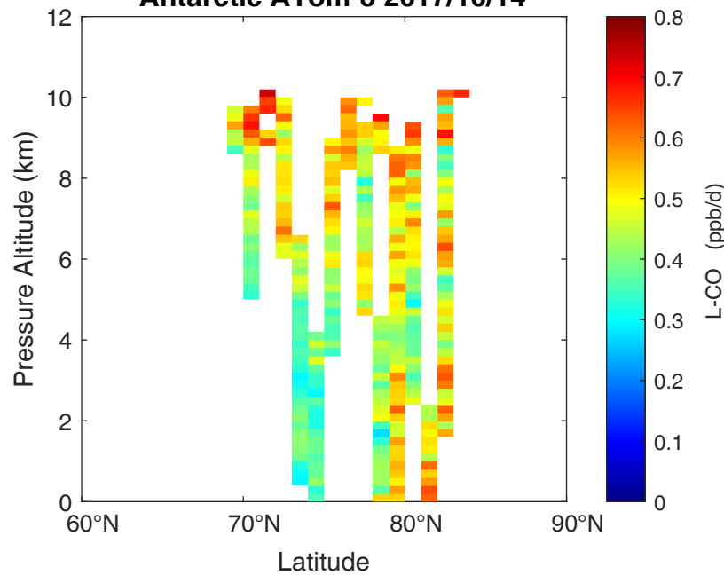
Antarctic ATom-3 2017/10/14
