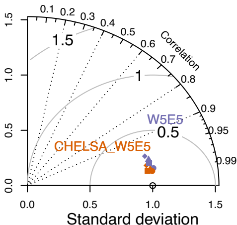
Maximum Daily 2m Air Temperature
