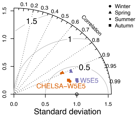
Monthly Shortwave Downwelling Radiation
