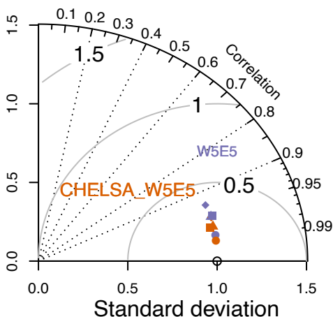
Monthly Shortwave Downwelling Radiation
