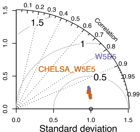
Mean Daily Precipitation
