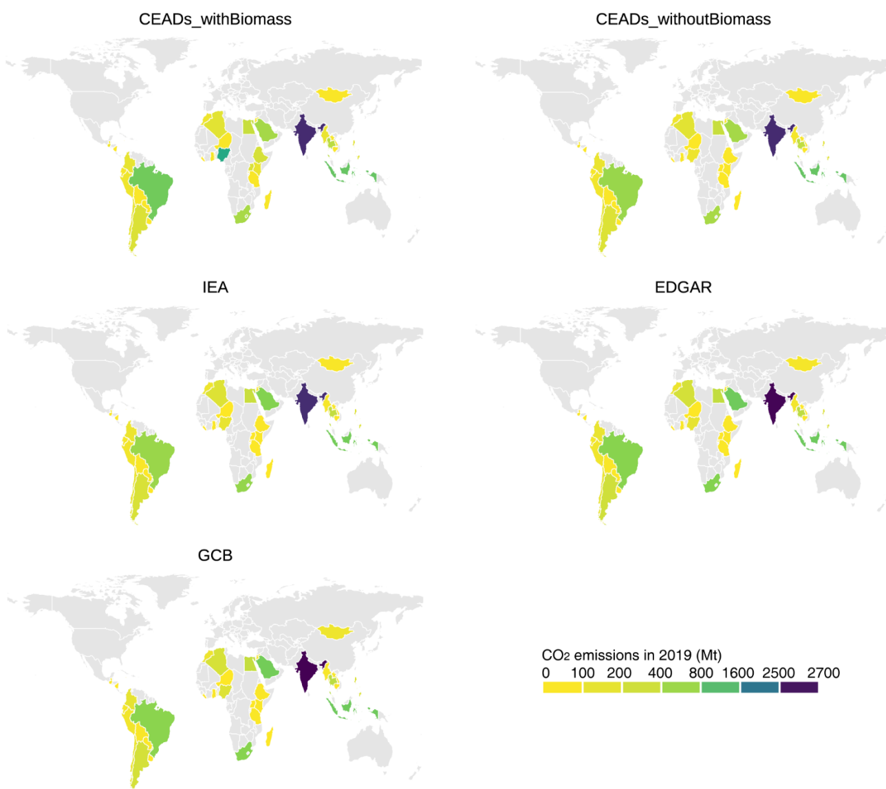
Figure S 2 Comparison of this dataset (CEADs with and without biomass) and IEA, EDGAR, and GCB.
