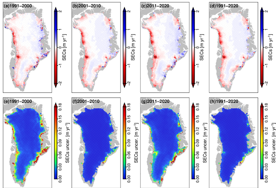
Figure 5. Maps of long-term SECs and their uncertainties from the combined elevation time series over the periods of (a, e) 1991–2000, (b, f) 2001–2010, (c, g) 2011–2020, and (d, h) 1991–2020.
