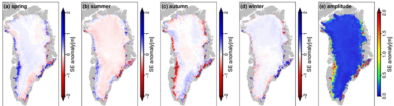
Figure 4. Climatological maps of the SE anomaly averaging season by season: (a) spring (January–February–March), (b) summer (April–May–June), (c) autumn (July–August–September), and (d) winter (October–November–December) and (e) the amplitude of corresponding annual variation over the periods of 1991–2020 from the merged elevation time series.
