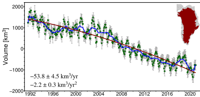
Figure 8. Volume change of the entire GrIS south of 81.5^{\circ} N from our merged altimetric time series (green dots) and its corresponding result after removing seasonal oscillations using a 13-month moving average (blue solid curve). The solid red line is the best-fit quadratic curve for the linear- and quadratic-trend estimates of volume change. The grey error bars show the 1\sigma uncertainty range of the altimetry data. The red-shaded area in the inset indicates the coverage of the GrIS with reference to the Greenland drainage system boundaries in Zwally et al. (2012).
