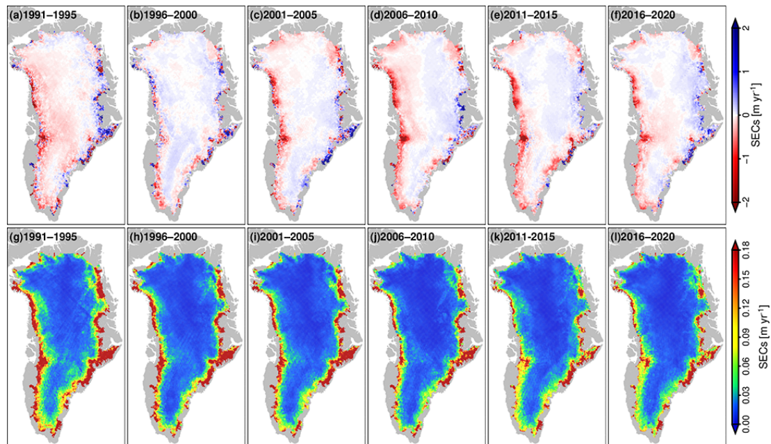
Figure 6. Maps of long-term SECs and their uncertainties from the combined elevation time series over the periods of (a, g) 1991–1995, (b, h) 1996–2000, (c, i) 2001–2005, (d, j) 2006–2010, (e, k) 2011–2015, and (f, l) 2016–2020.
