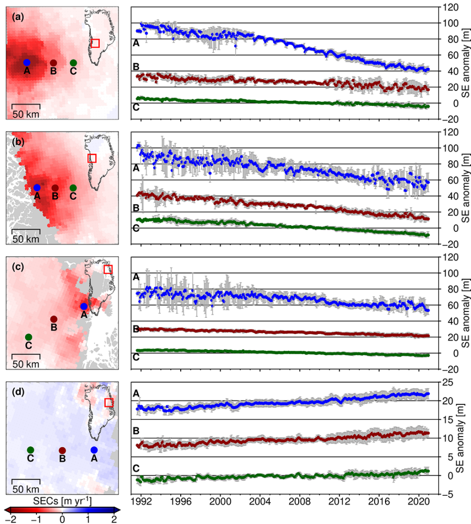
Figure 7. SE anomaly time series near (a) Jakobshavn Isbræ, (b) Upernavik Isstrøm, (c) Zachariæ Isstrøm and Nioghalvfjærdsfjorden Glacier, and (d) King Christian X Land. The locations of the selected points (A, B, and C) are marked in the left-hand maps of elevation change over 1991–2020. The time series and the 1\sigma uncertainty ranges for each point are given in the right-hand plots with the time series of points A and B shifted along the SE anomaly axis for better visibility.
