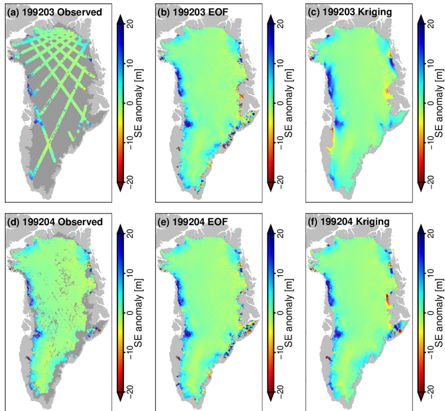
Figure 3. Interpolation performance of EOF reconstruction and ordinary kriging: panels (a), (b), and (c) are the results for the March 1992 (199203) observation, EOF reconstruction, and ordinary kriging interpolation, respectively, and panels (d), (e), and (f) are the same for April 1992 (199204).
