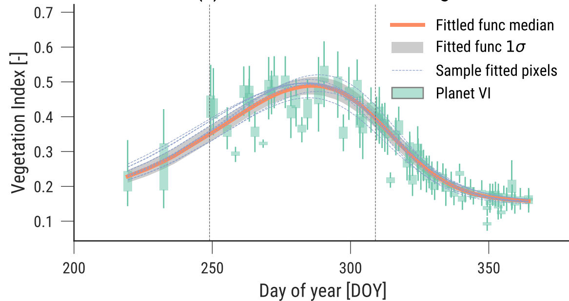
(c) Constrained model fitting
