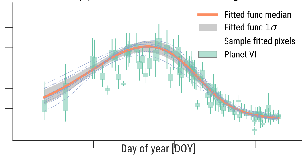
(b) Unconstrained model fitting
