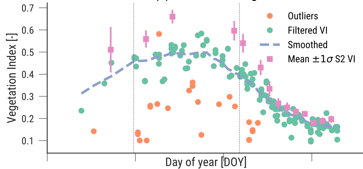
(c) Constrained model fitting
