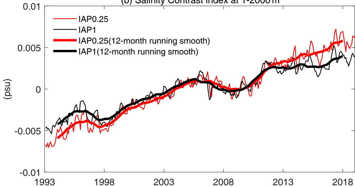
(b) Salinity Contrast index at 1-2000 m
