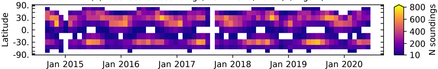
(b) N collocated soundings, 2014-2020, Land (H/M gain)
