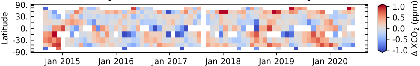
(a) \Delta XCO_2 (GOSAT v9 - OCO2 v10), 2014-2020, Land (H/M gain)
