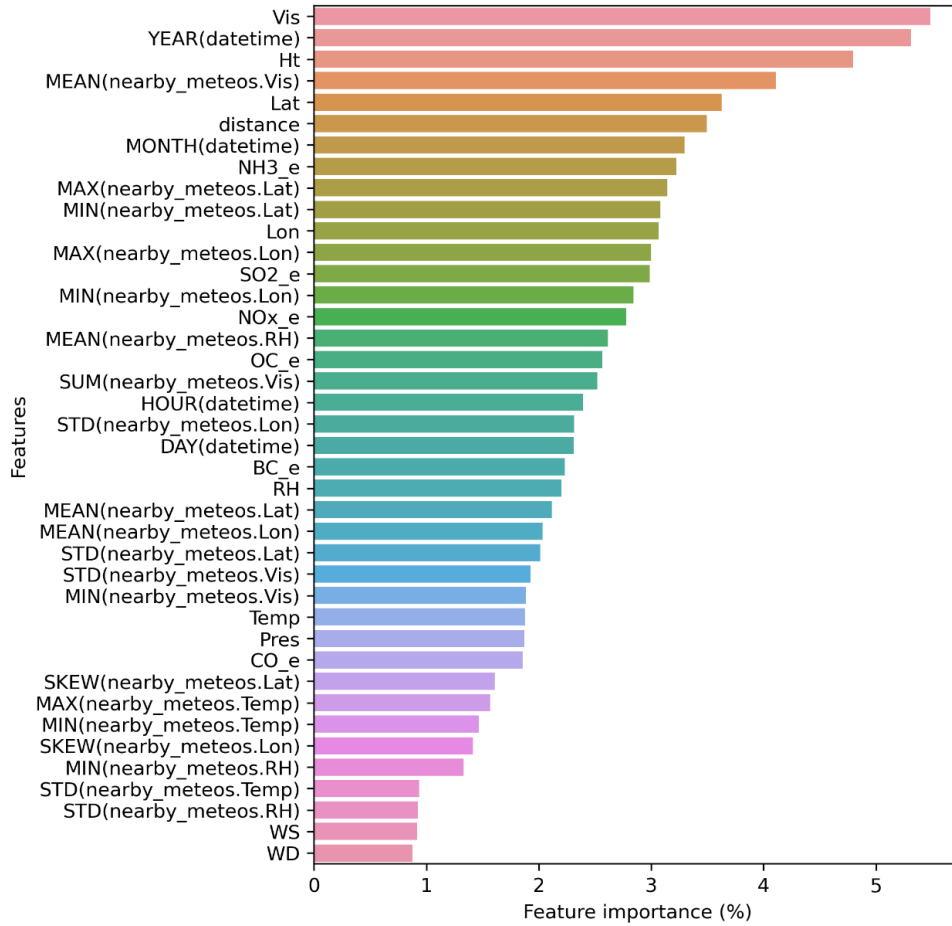
Fig. S1 Relative importance of all the features used in our model
