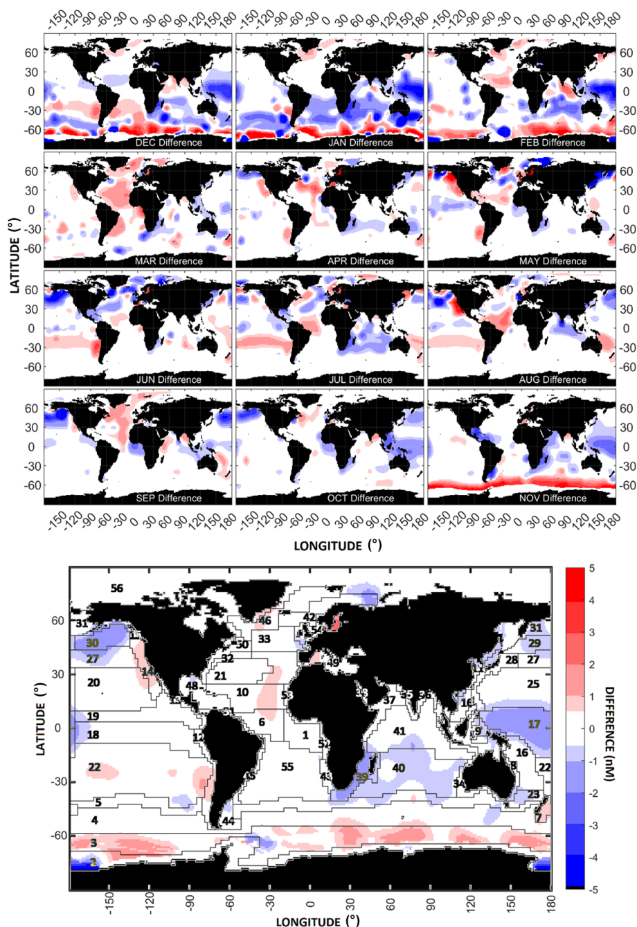
Figure 9. Differences between the monthly and annual mean DMS concentrations of the Rev3 and L11 climatologies (Rev3 – L11).
