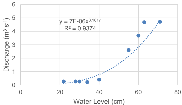
Querococha Rating Curve
