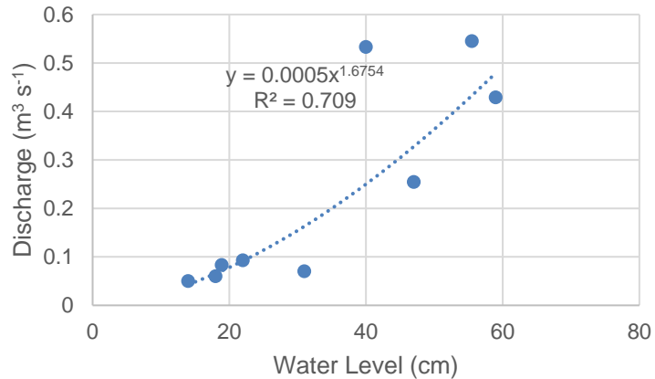
Cuchillacocha Rating Curve
