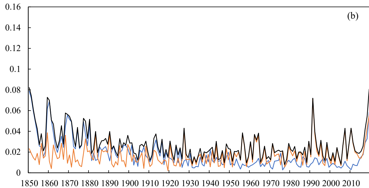
Reconstructed C-LSAT2.0 + I max (65°N-90°N)
