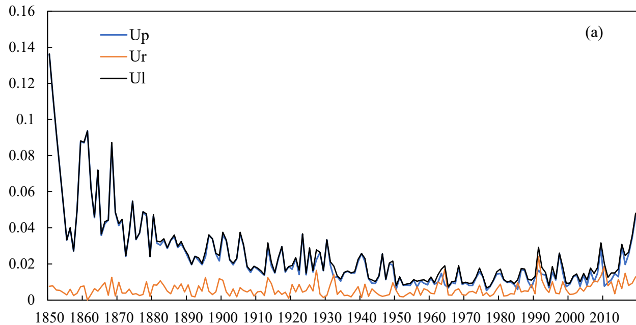
Reconstructed C-LSAT2.0 + I min (80°N-90°N)
