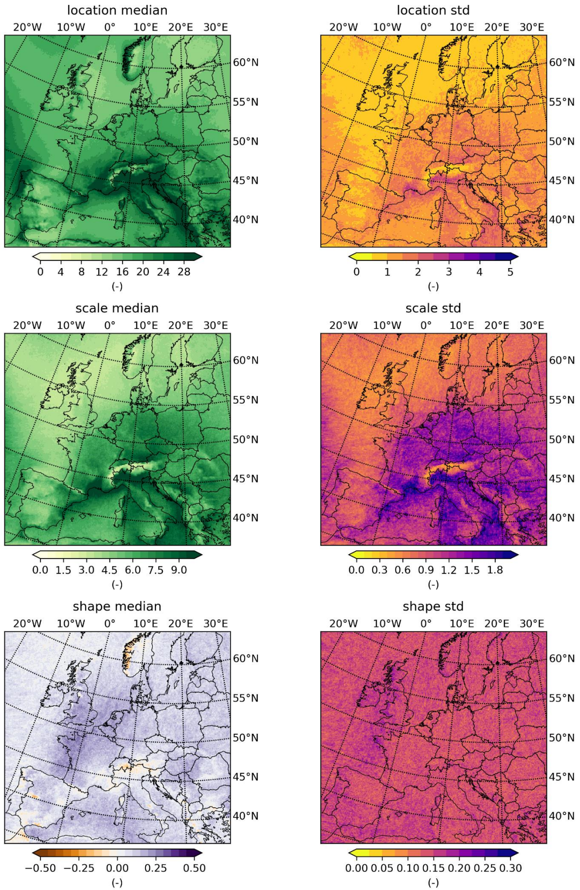
Figure S1: Median and standard deviation (std) of the three GEV parameters regarding the 50 CRCM5-LE members.
