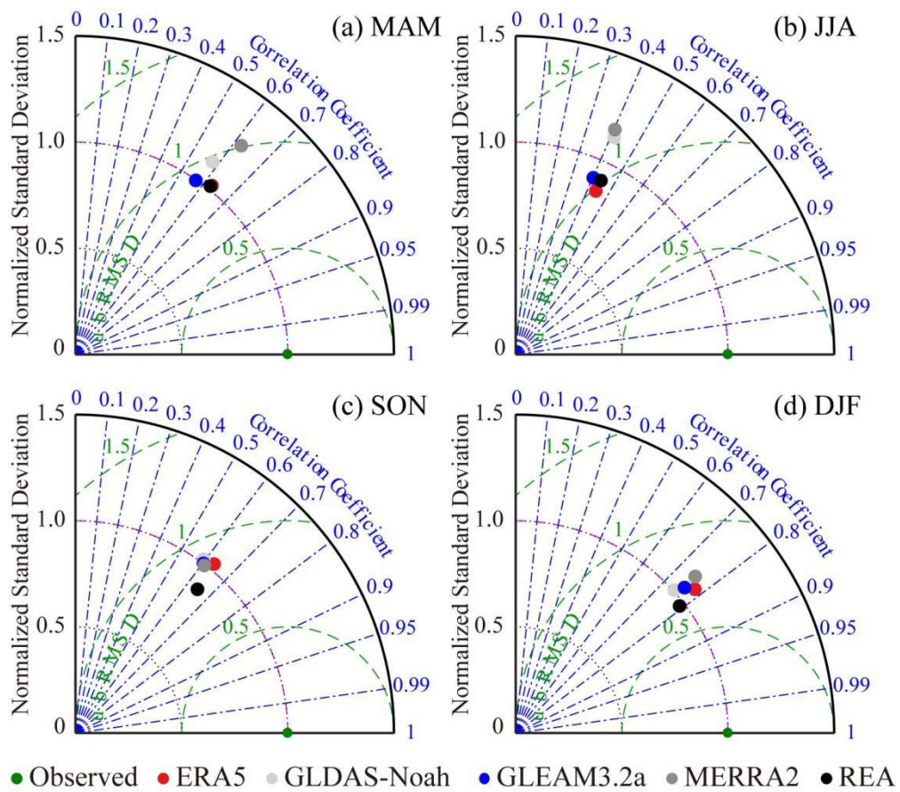
Figure S4. Taylor diagrams of daily Ground-measured ET and ET from different products in different seasons.
