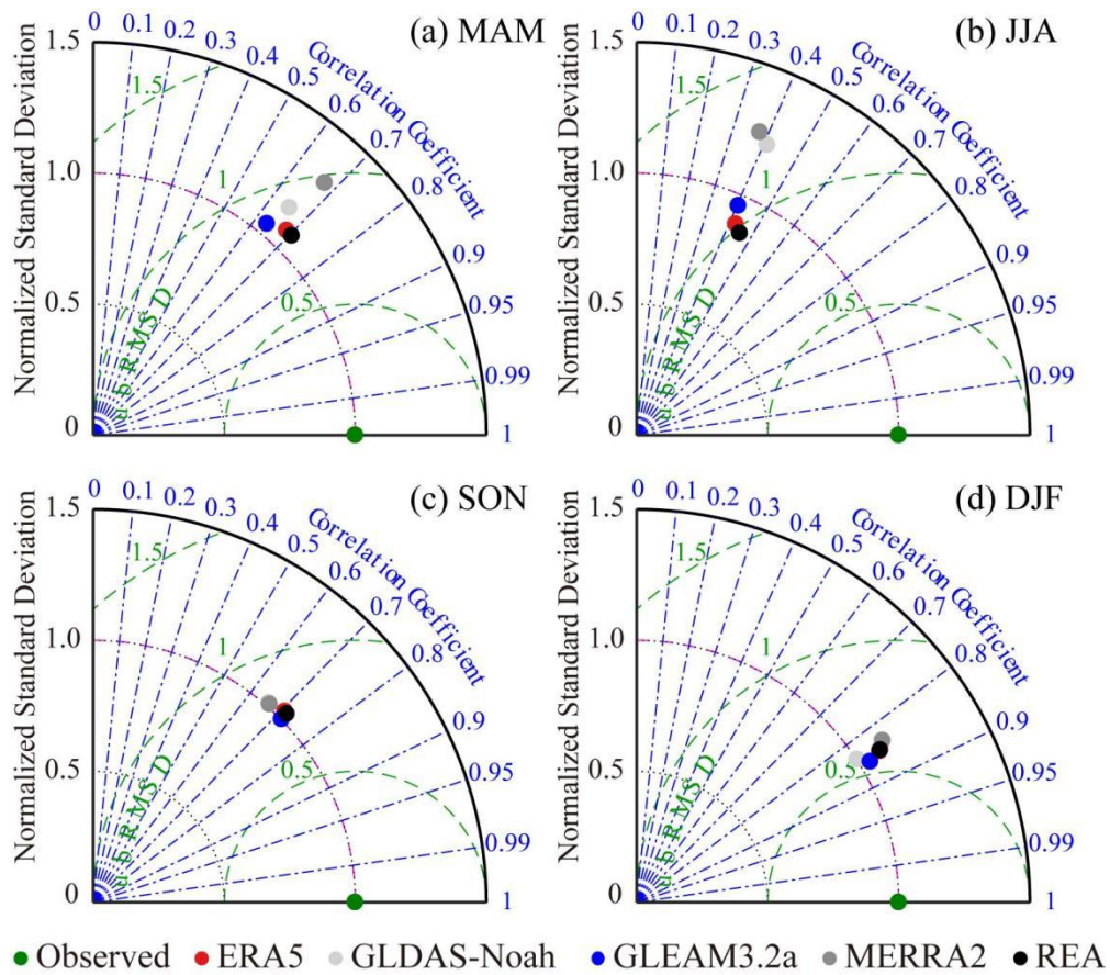
Figure S5. Taylor diagrams of monthly Ground-measured ET and ET from different products in different seasons.
