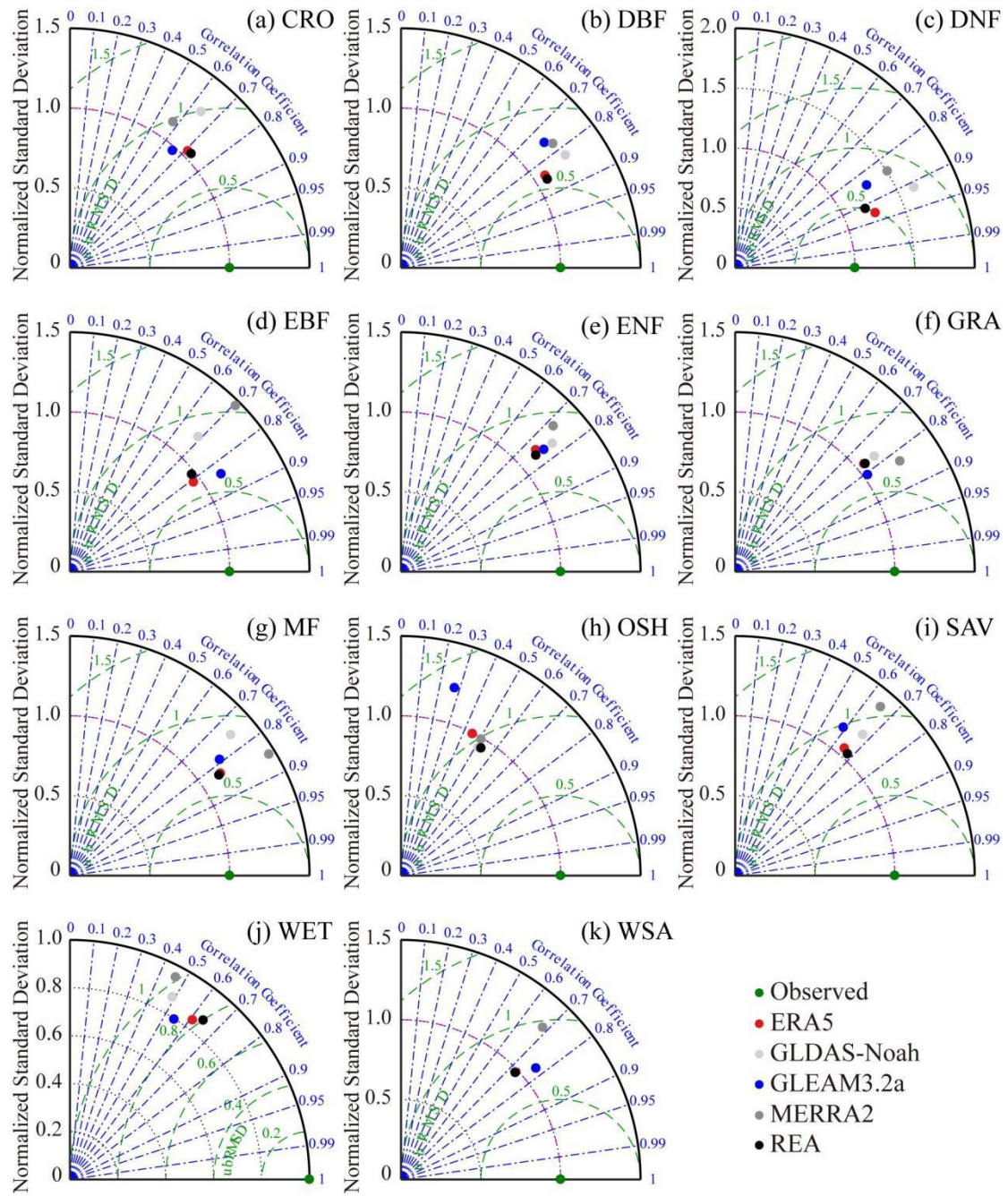
Figure S3. Taylor diagrams of monthly Ground-measure ET and ET from the different products in different ecosystems.
