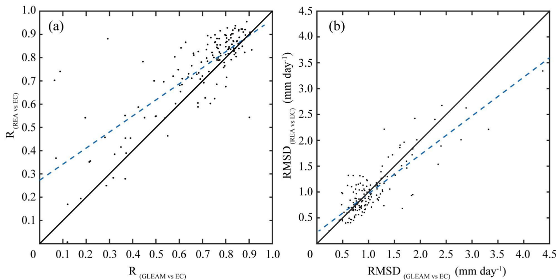
Figure S6. Scatter plots of the correlation coefficients and RMSD between GLEAM, REA and Ground-measured ET. Linear fits are plotted in blue and the 1:1 line is depicted.
