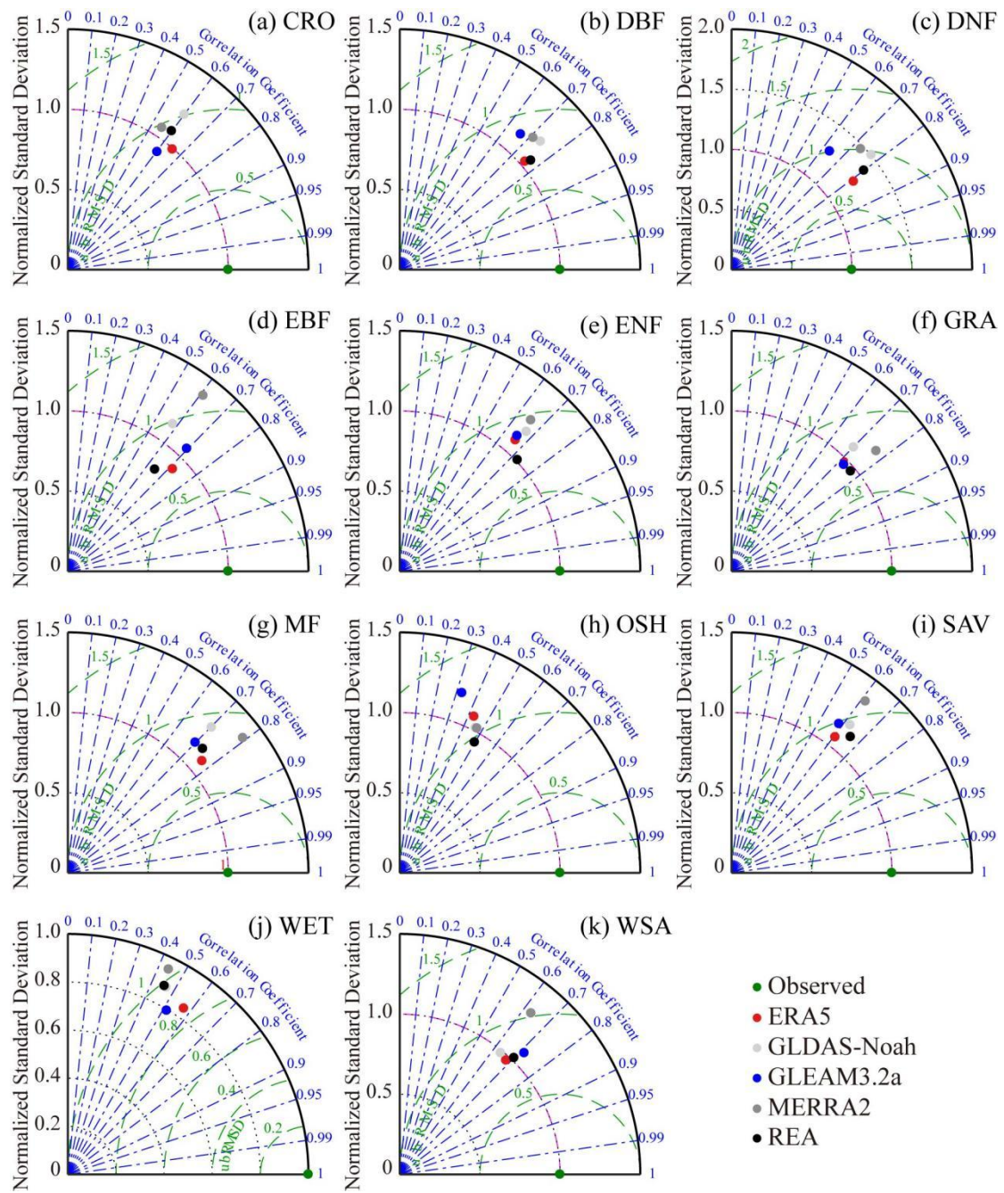
Figure S2. Taylor diagrams of daily Ground-measure ET and ET from different products in different ecosystems.
