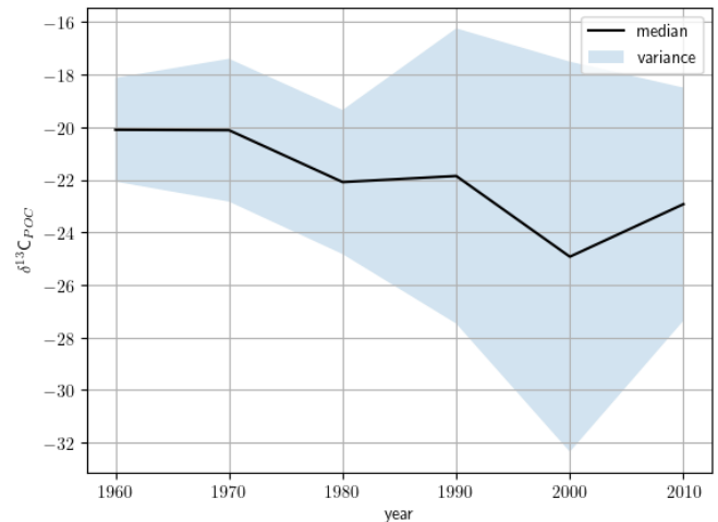
Figure 12. The decadal shift in \delta^{13}\text{C}_{\text{POC}} values in the uppermost 130 m for all but the Southern Ocean: \delta^{13}\text{C}_{\text{POC}} decadal median against the decades. The shaded area around the graph marks the variance of the respective decade in each direction.
