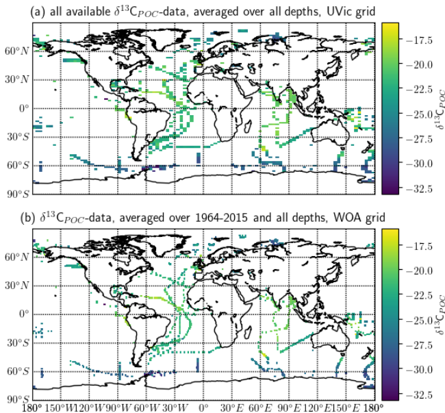
Figure 6. Global distribution of the \delta^{13}\text{C}_{\text{POC}} data is visualized based on the (a) UVic grid and (b) WOA grid. The data used for (a) are independent of time and include all available measurements with latitude and longitude information. The data shown in (b) include only data with complete temporal metadata and are averaged over the years 1964–2015. Both kinds of data are averaged over all measurements including data with missing depth information. Each colored square refers to a grid cell with available \delta^{13}\text{C}_{\text{POC}} measurements. The colors indicate the \delta^{13}\text{C}_{\text{POC}} value in the respective grid cell.
