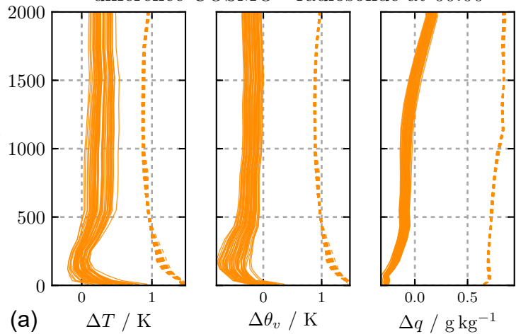
difference COSMO - radiosonde at 00:00
