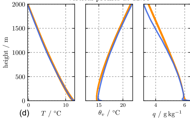
vertical profiles at 12:00
