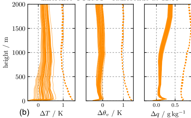
difference COSMO - radiosonde at 12:00
