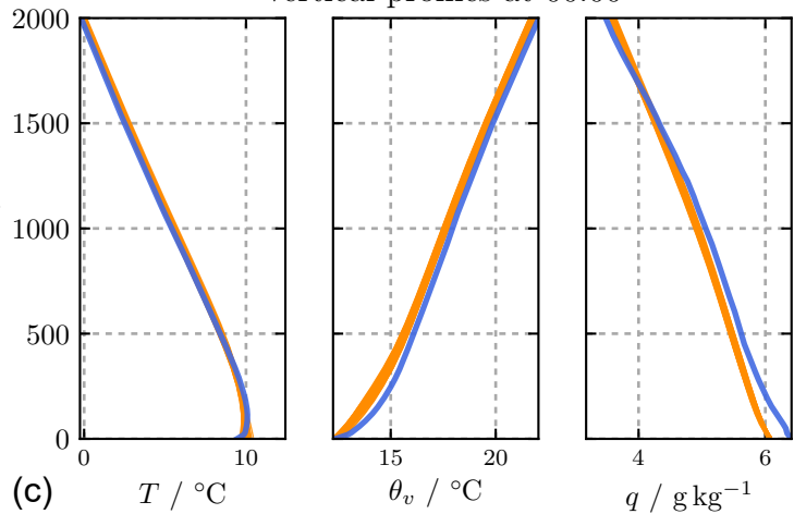
vertical profiles at 00:00
