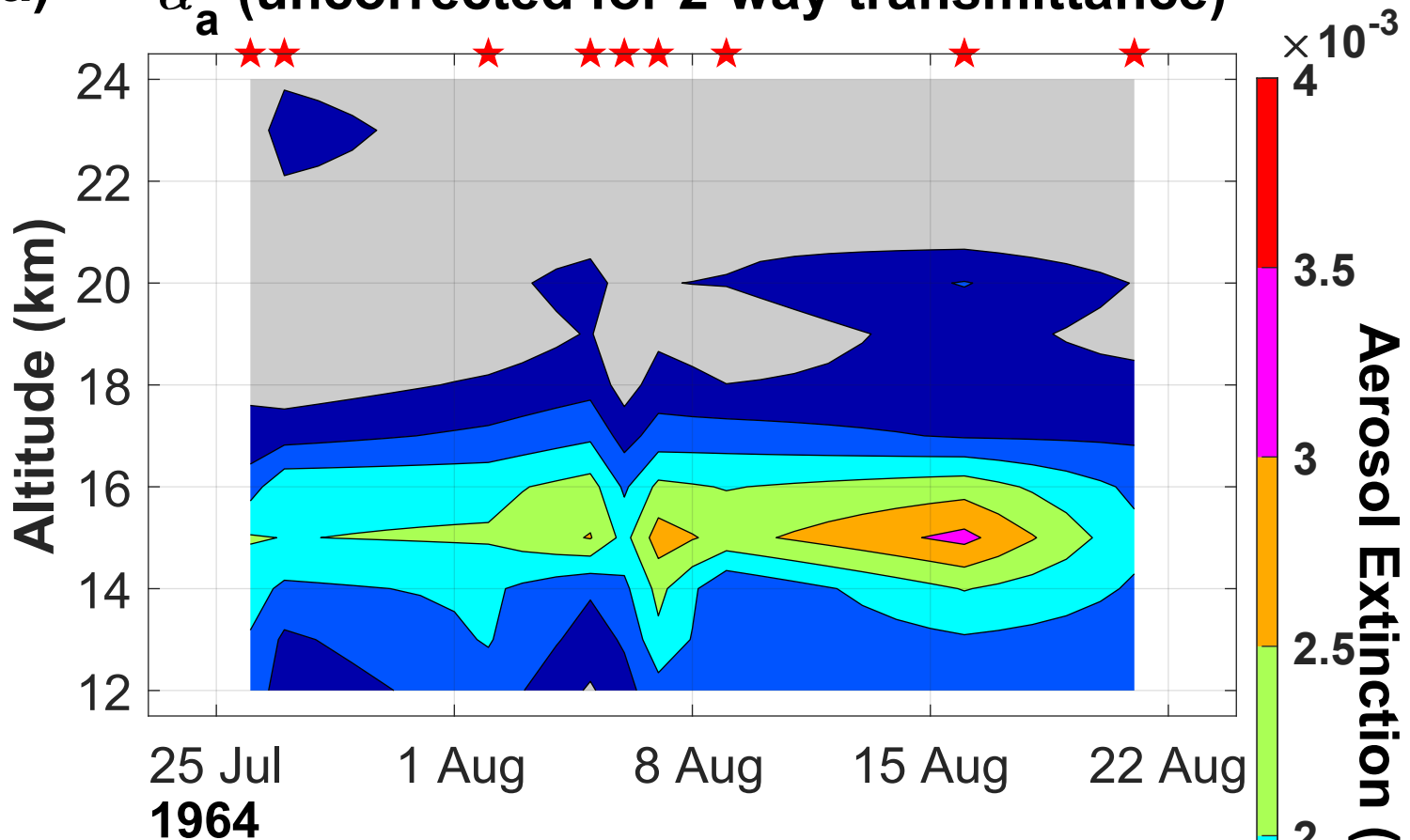
(a) \alpha_a (uncorrected for 2-way transmittance)
