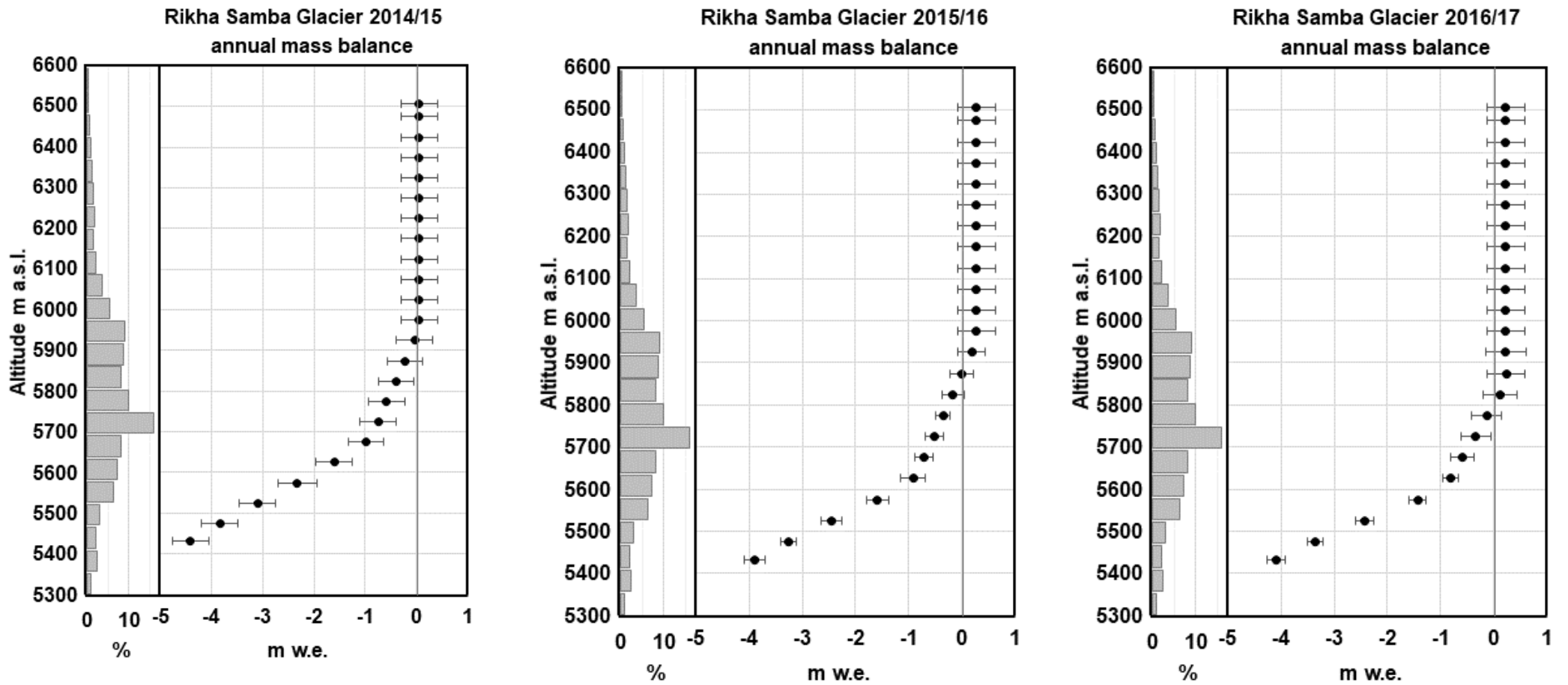
Figure S6: The annual mass balances and uncertainties for 50 m elevation bands of Rikha Samba Glacier for the mass-balance years 2014/15, 2015/16 and 2016/17.
