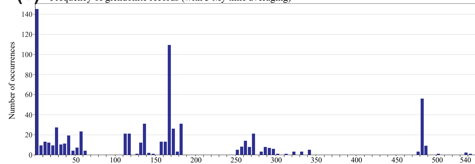
(c) Frequency of glendonite records (with 5 My time averaging)
