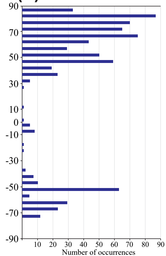
(b) Latitudinal frequency (5° averaging)
