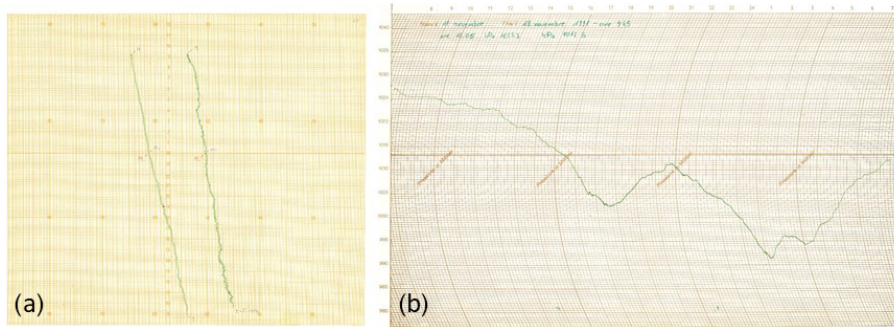
Figure 2. (a) Sprung-Fuess barograph chart from 2 February 1954 at 10:00 to 4 February 1954 at 09:00. (b) Fuess 87M barograph chart from 11 November 1991 at 10:05 to 18 November 1991 at 09:45.
