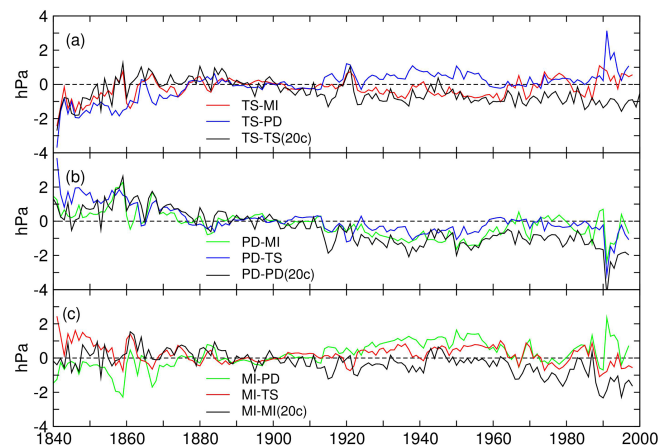
Figure 7. Comparisons of annual mean pressures (hPa): (a) differences involving Trieste (TS); (b) differences involving Padua (PD); and (c) differences involving Milan (MI). Black curves represent the comparisons between each station and the corresponding time series from the 20th Century Reanalysis (20c); the comparison between Trieste and Milan is shown in red, that between Trieste and Padua in blue, and that between Padua and Milan in green.
