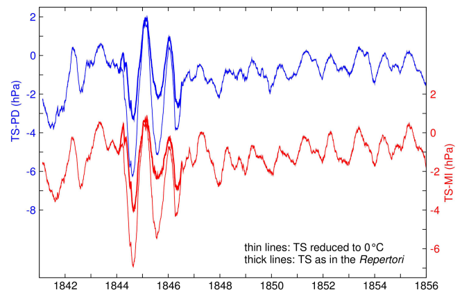
Figure 6. 91 d running means of daily mean-sea-level pressure differences between Trieste (TS) and Padua (PD) (blue curves, left scale) and between Trieste and Milan (MI) (red curves, right scale). The thin lines correspond to Trieste pressure reduced to 0^\circ\text{C} , and the thick lines correspond to Trieste pressure from 10 March 1844 to 23 May 1846 as it appears in the Repertori .
