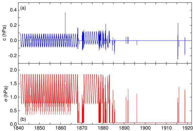
Figure 3. Daily corrections ( c , panel a) and errors ( \sigma , panel b) from 1841 to 1920 in hectopascals. From 1920 onwards, c = 0 hPa and \sigma = 0.06 hPa.
