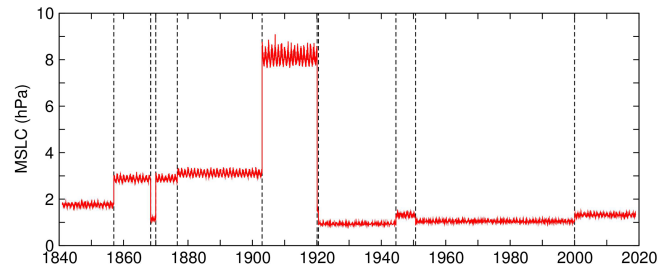
Figure A1. Daily corrections to reduce pressure to MSL (MSLC) in hectopascals. The dashed vertical lines correspond to the barometer height changes summarized in Table 3.
