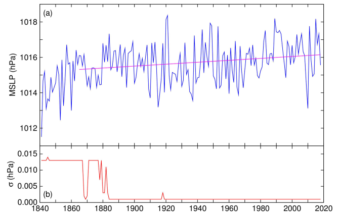
Figure 5. Annual mean-sea-level pressure (MSLP, panel a) and errors ( \sigma , panel b) in hectopascals. The 1865–2018 linear trend of 0.5 \pm 0.2 hPa per century is shown (magenta line).
