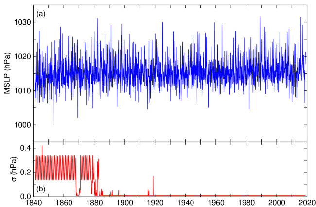
Figure 4. Monthly mean-sea-level pressure (MSLP, panel a) and errors ( \sigma , panel b) in hectopascals.
