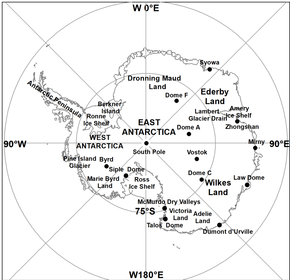
Fig S1: Map of Antarctic Ice Sheet showing the main locations presented in the text
