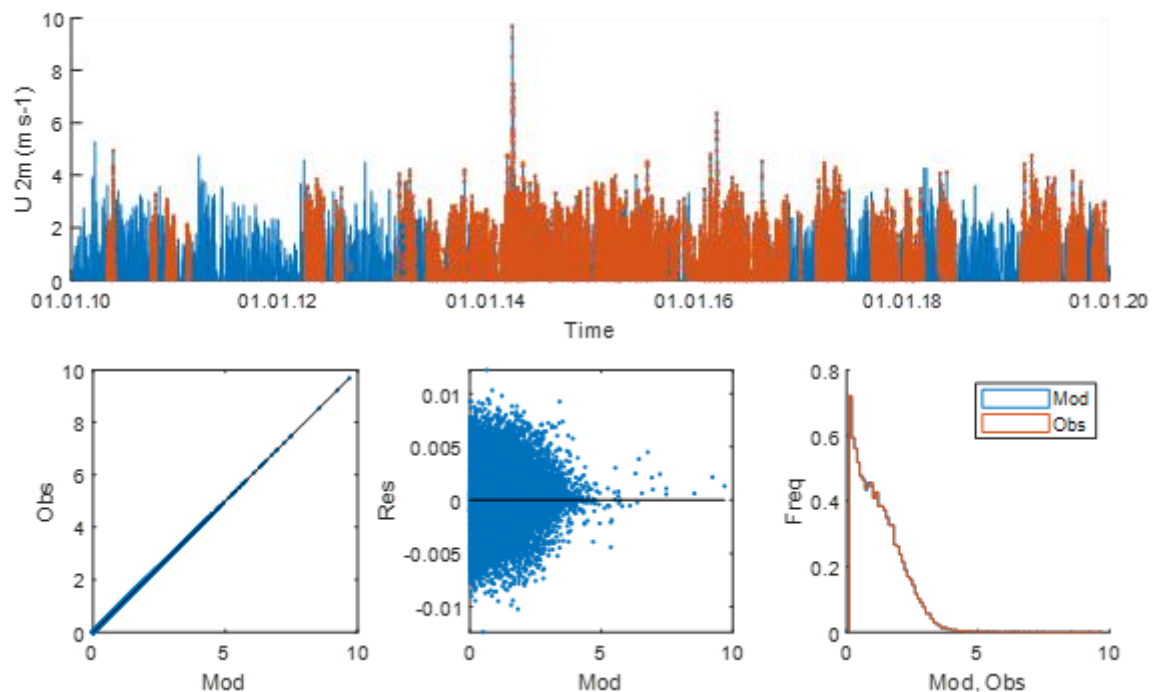
55 Figure S14. U-wind component at 2 m above the hollow surface at the MFS. See legend at Fig. S1.
