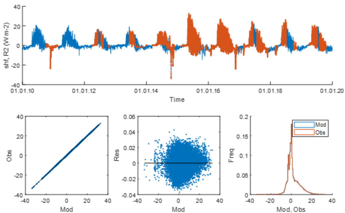
Figure S13. Soil heat flux at the ridge (site 2) at the MFS. See legend at Fig. S1.
