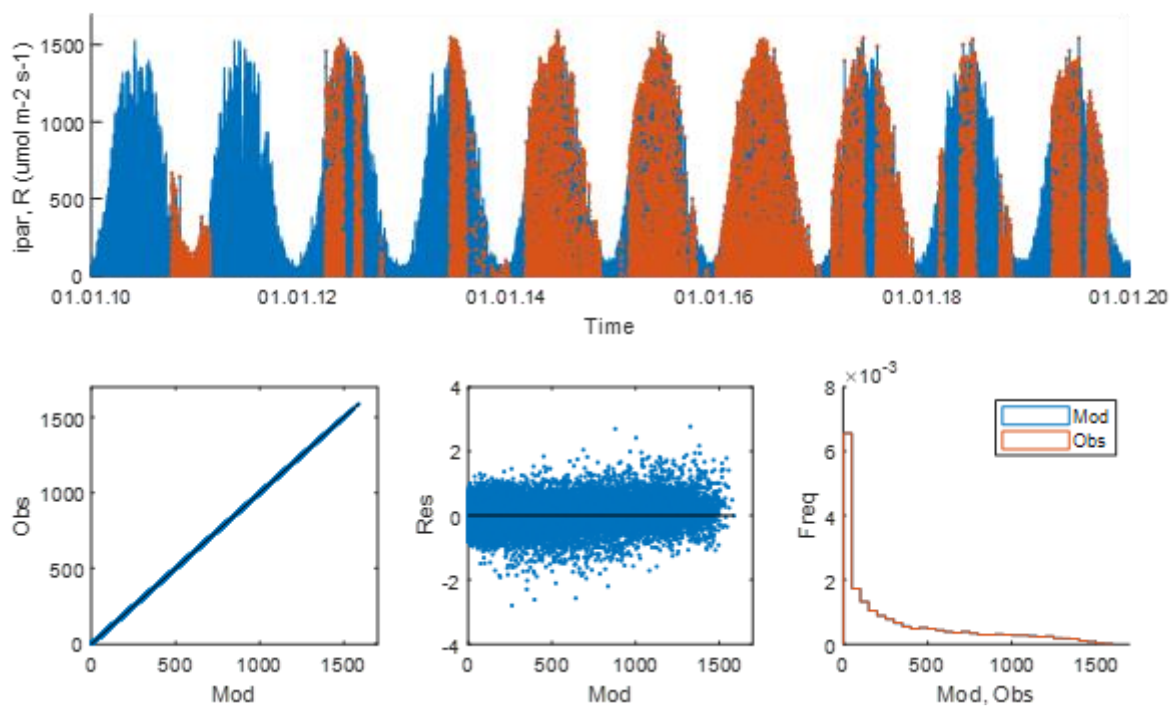
Figure S6. Incoming photosynthetically active radiation at the ridge at the MFS. See legend at Fig. S1.
