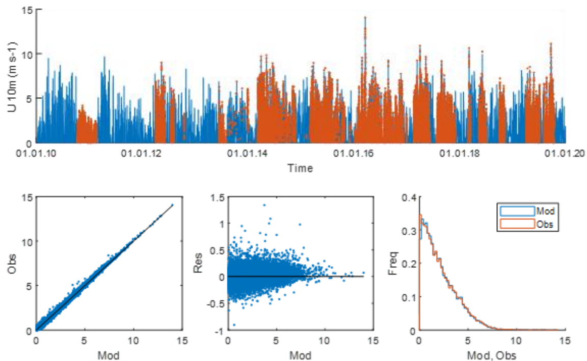
Figure S16. U-wind component at 10 m above the ridge surface at the MFS. See legend at Fig. S1.
