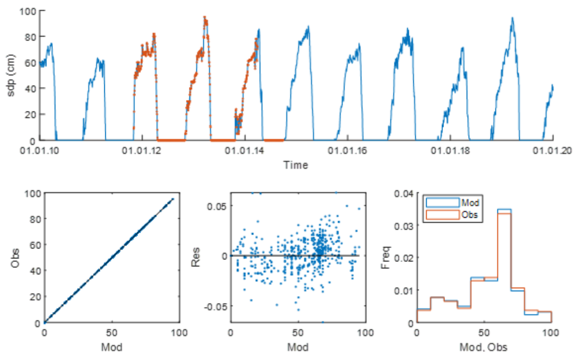
70 Figure S19. Snow depth at the hollow at the MFS. See legend at Fig. S1.
