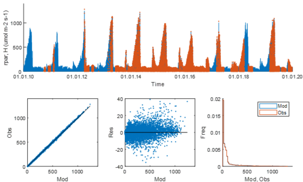
Figure S7. Reflected photosynthetically active radiation at the hollow at the MFS. See legend at Fig. S1.
