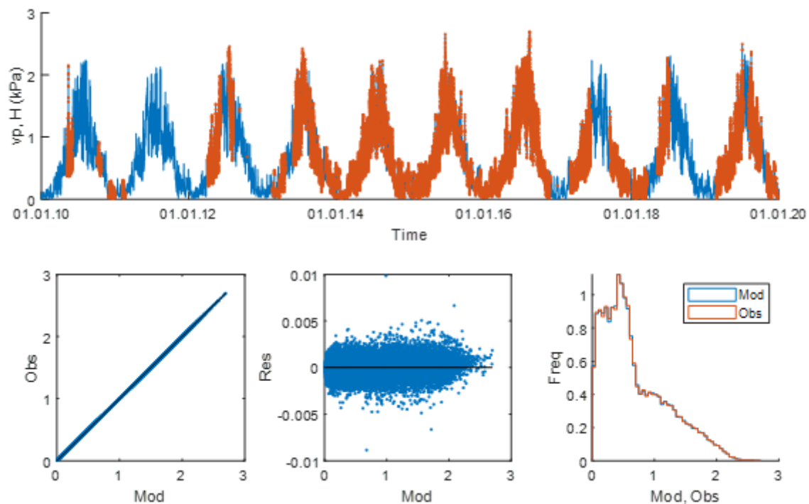
20 Figure S3. Water vapour pressure at the hollow at the MFS. See legend at Fig. S1.
