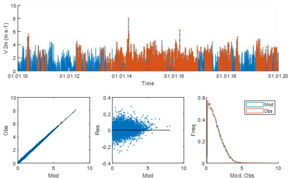
Figure S15. V-wind component at 2 m above the hollow surface at the MFS. See legend at Fig. S1.
