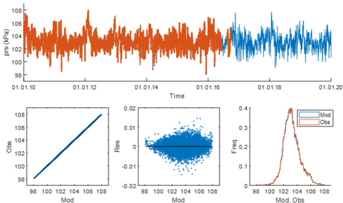
Figure S18. Atmospheric pressure at the MFS. See legend at Fig. S1.
