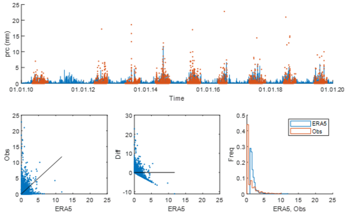
Figure S20. Liquid precipitations at the MFS. Top panel: Obs – hourly observations using rain gauge, ERA5 – ERA5-Land reanalysis data. Bottom panel: relations of observed and ERA5-Land data (left), difference of ERA5-Land with observation data (centre), frequency distributions for ERA5-Land and observed data (right).
