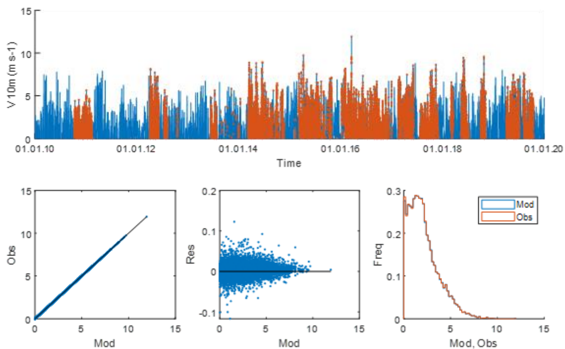
Figure S17. V-wind component at 10 m above the ridge surface at the MFS. See legend at Fig. S1.
