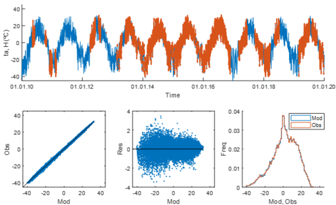
5 Figure S1. Air temperature measured at the hollow at the Mukhrino field station.
