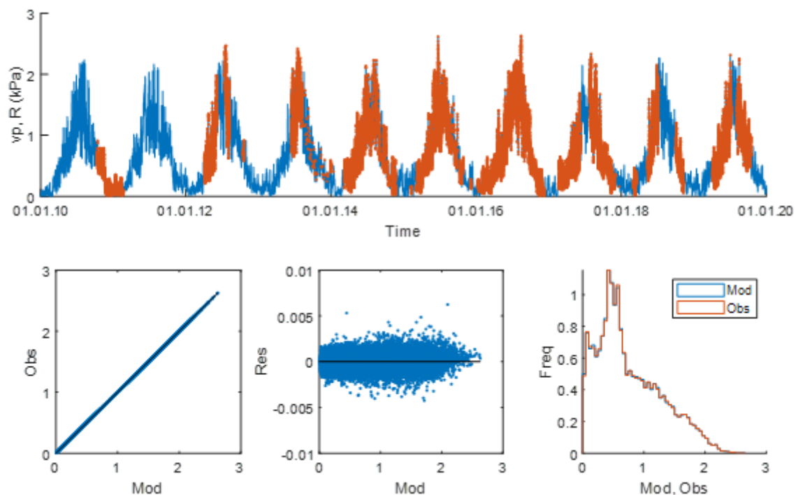
Figure S4. Water vapour pressure at the ridge at the MFS. See legend at Fig. S1.
