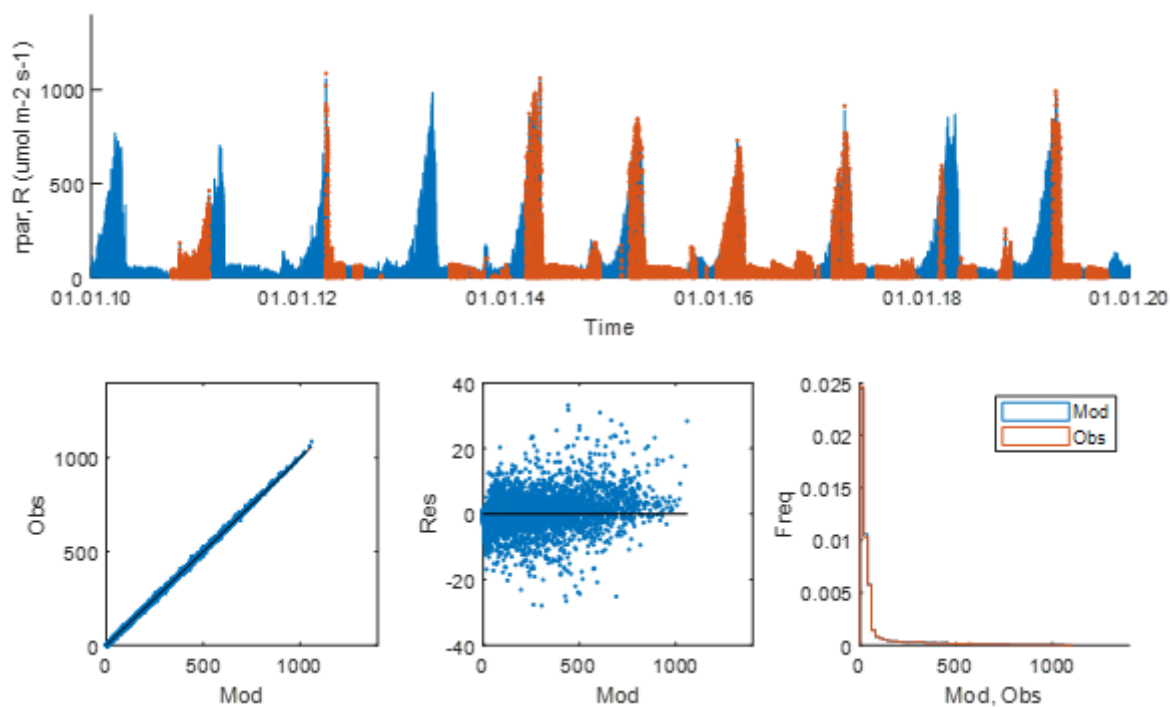
35 Figure S8. Reflected photosynthetically active radiation at the ridge at the MFS. See legend at Fig. S1.
