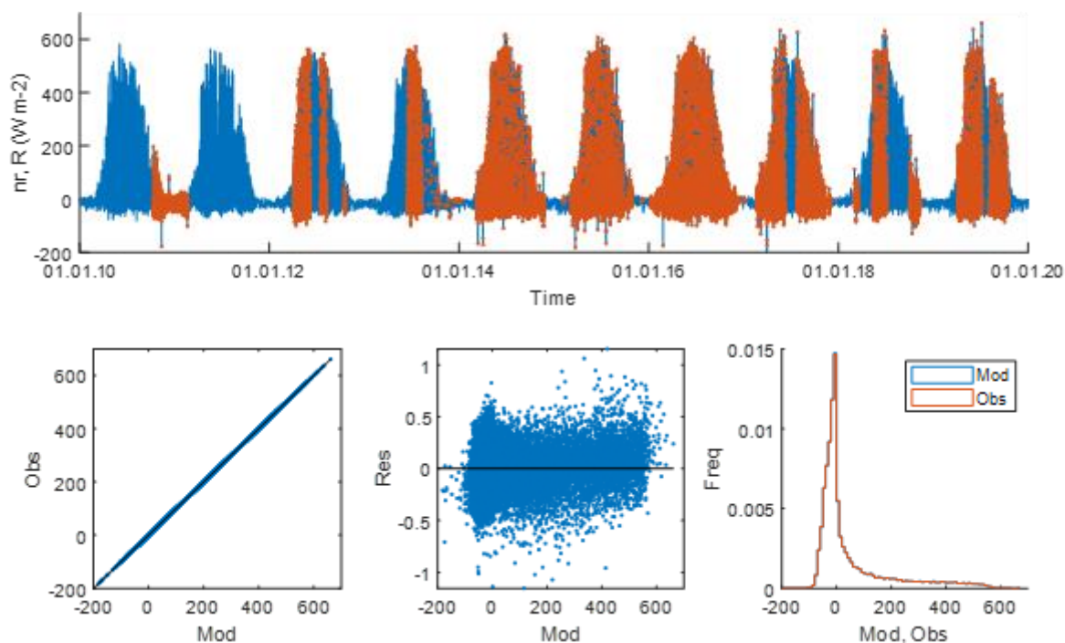
Figure S10. Net radiation balance at the ridge at the MFS. See legend at Fig. S1.
