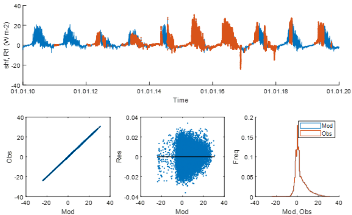
Figure S12. Soil heat flux at the ridge (site 1) at the MFS. See legend at Fig. S1.
