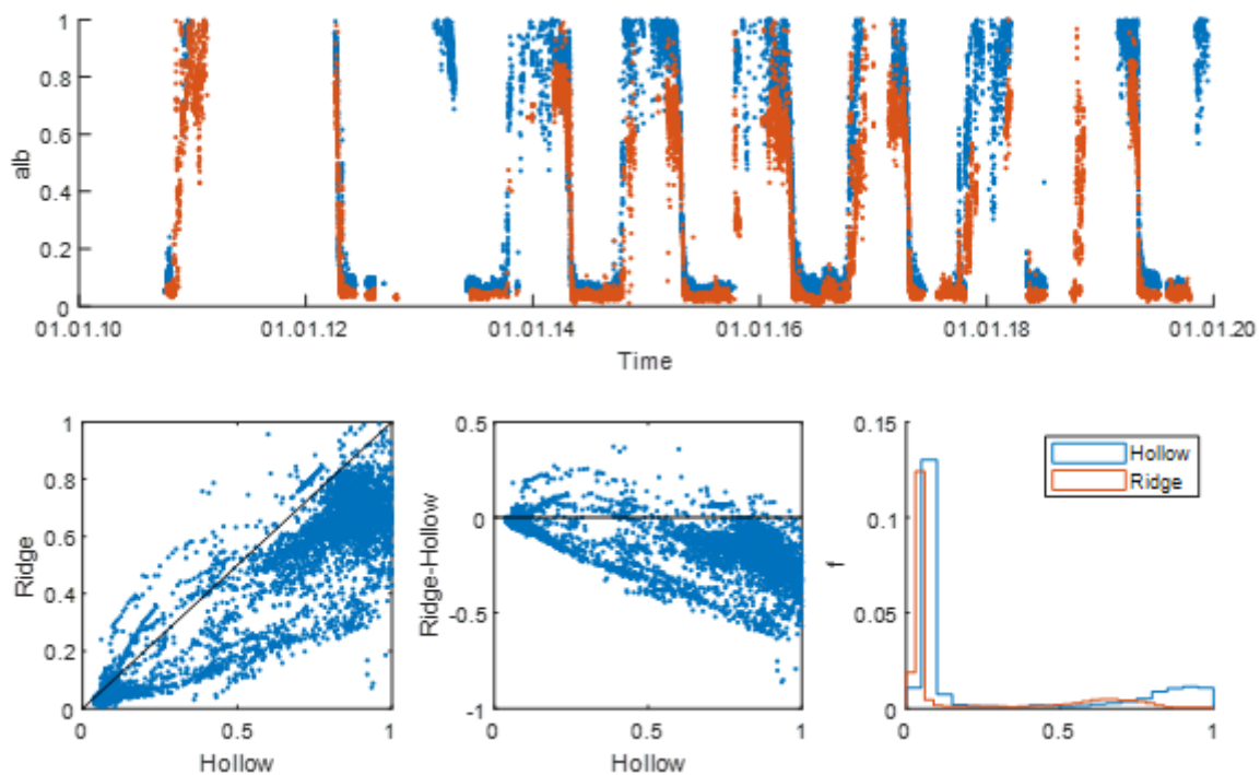
Figure S21. Albedo calculated from observations of incoming and reflected PAR at the MFS. Top panel: 1 – hollow, 2 – ridge. Bottom panel: data relations (left), difference of albedo at two sites (centre), frequency distributions (right).
