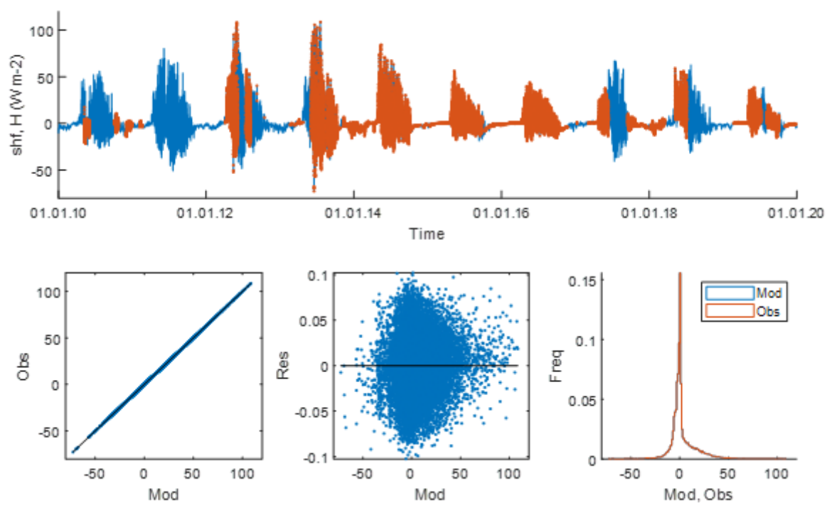
Figure S11. Soil heat flux at the hollow at the MFS. See legend at Fig. S1.
