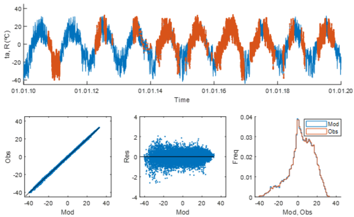
15 Figure S2. Air temperature at the ridge at the MFS. See legend at Fig. S1.
