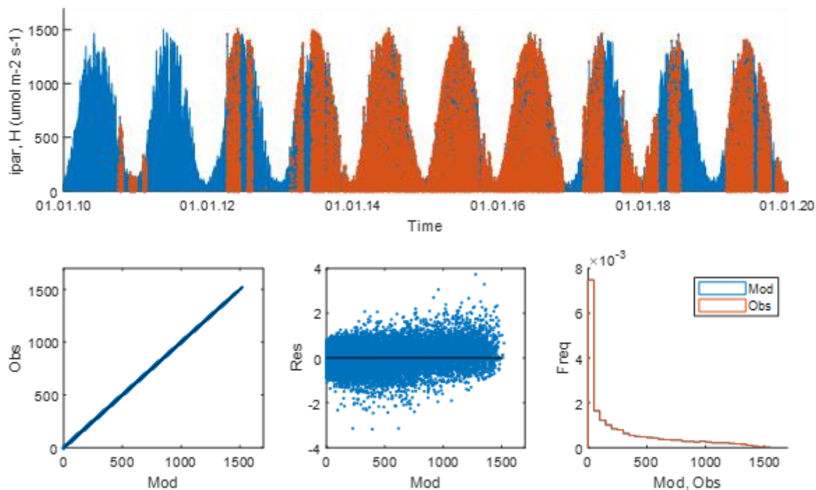
Figure S5. Incoming photosynthetically active radiation at the hollow at the MFS. See legend at Fig. S1.
