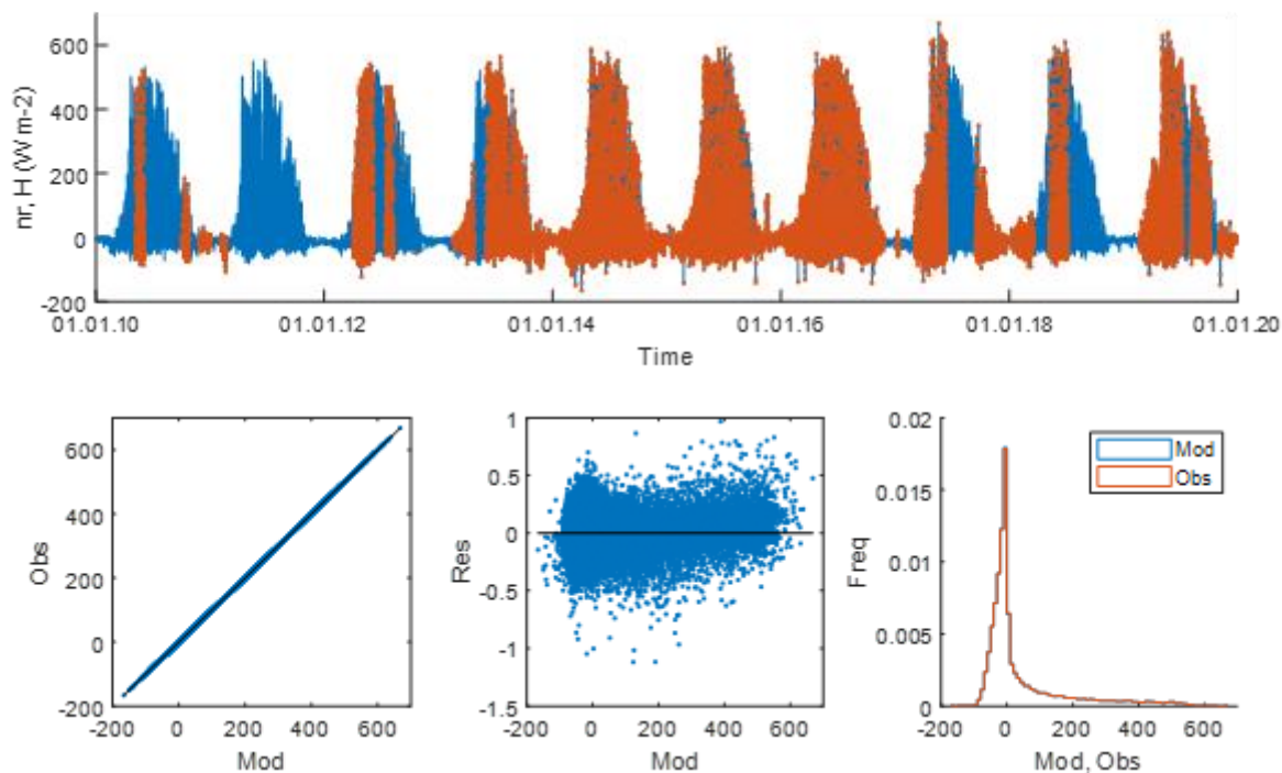
Figure S9. Net radiation balance at the hollow at the MFS. See legend at Fig. S1.
