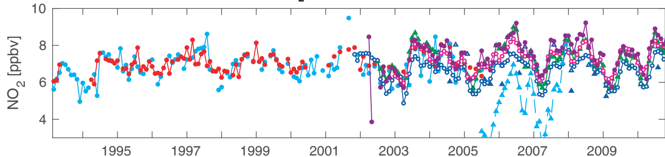
(a) \text{NO}_2 [ppbv] 20°S-20°N, 10 hPa
