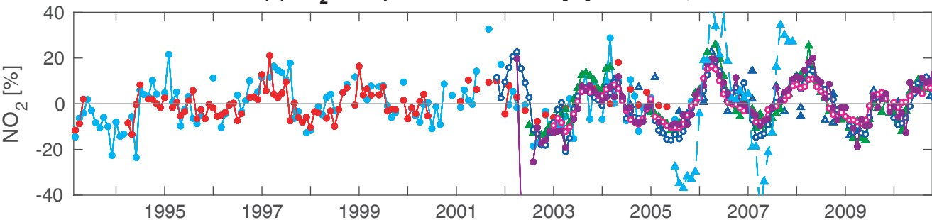
(b) \text{NO}_2 multiplicative anomalies [%] 20°S-20°N, 10 hPa
