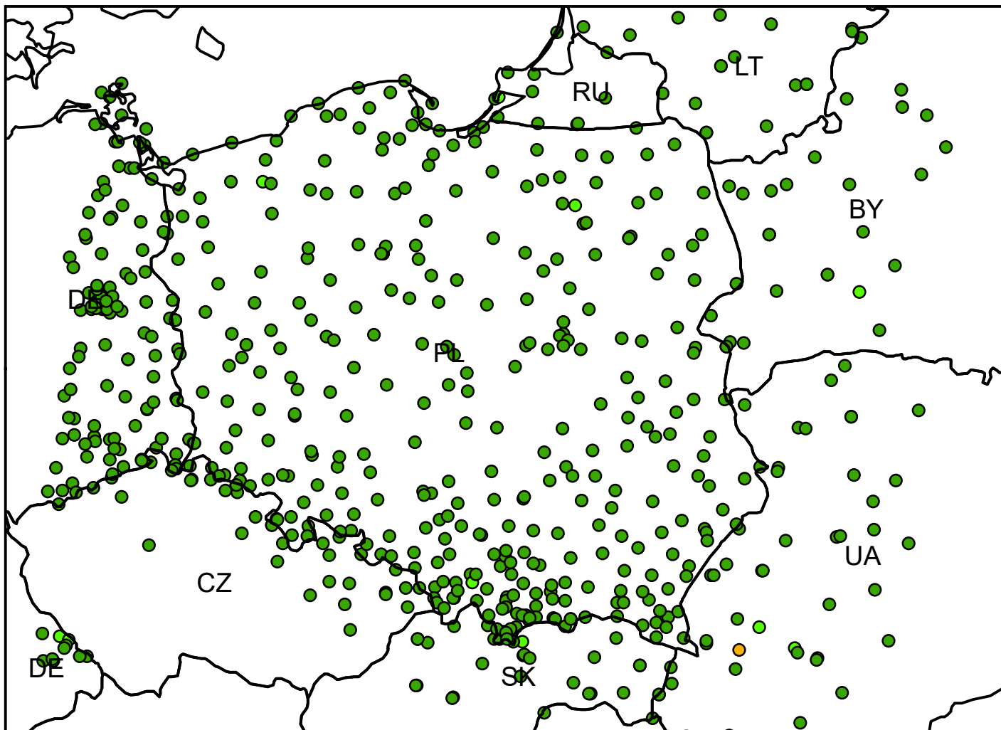
Correlation for minimum temperature stations
