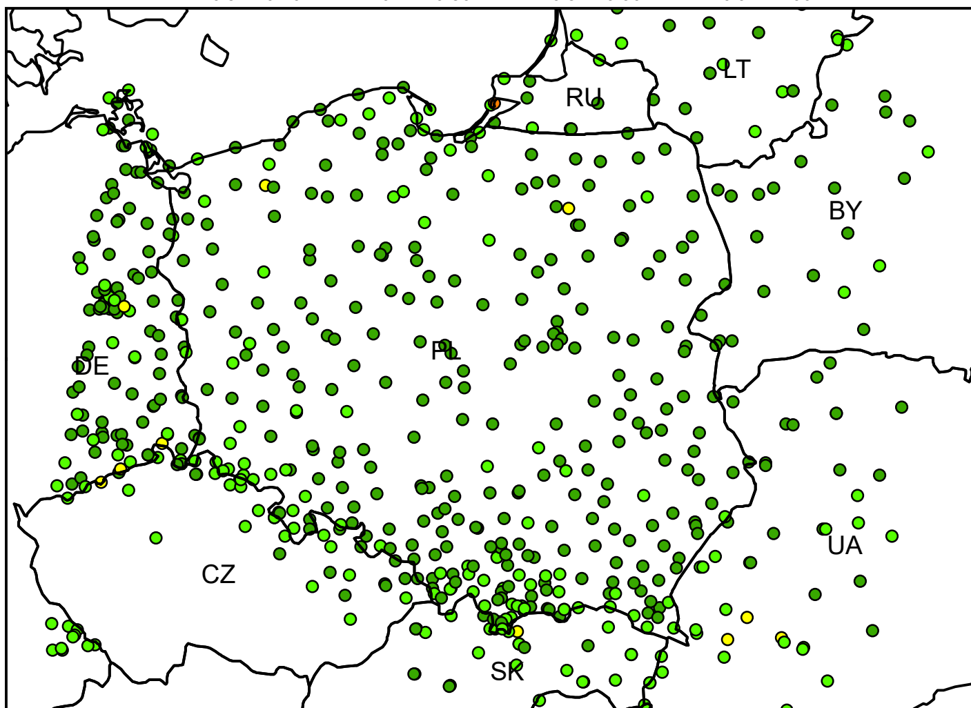
RMSEsd for minimum temperature stations
