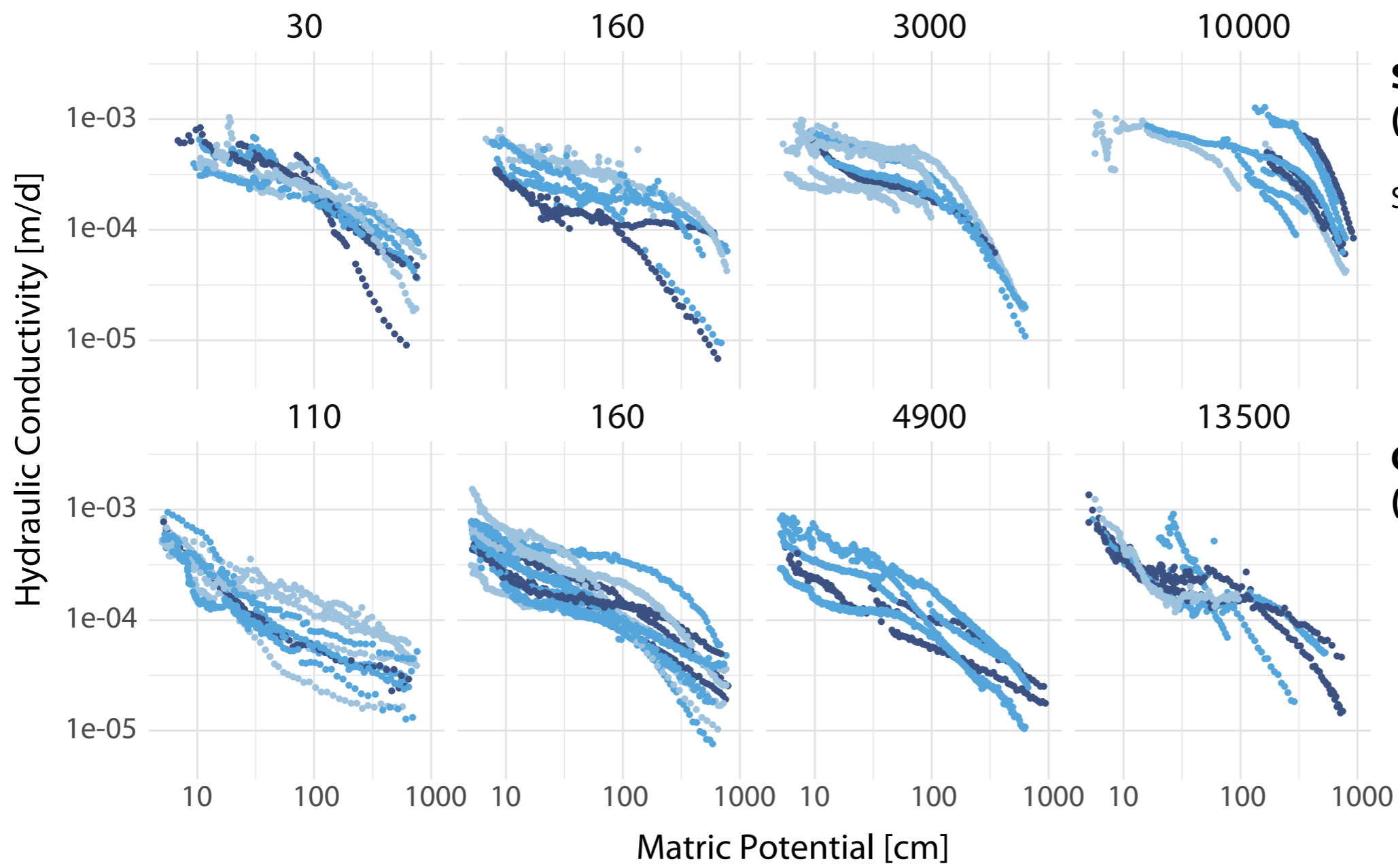
(b) Conductivity curves sorted by moraine age [years]
