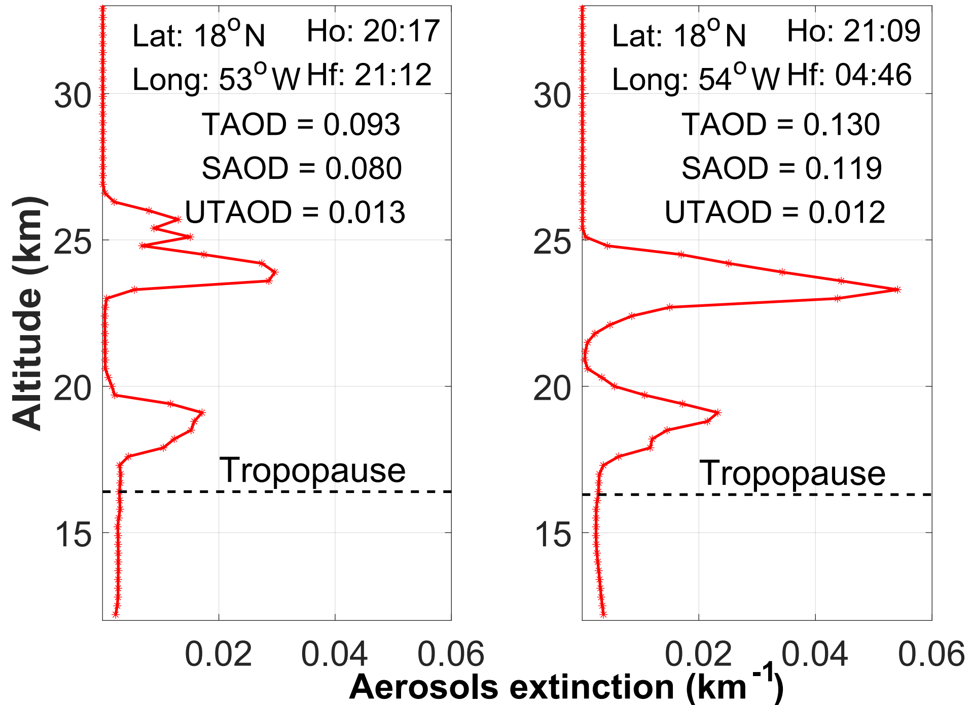
(a) 19910803 Day: 215.8 (b) 19910804 Day: 216.9
