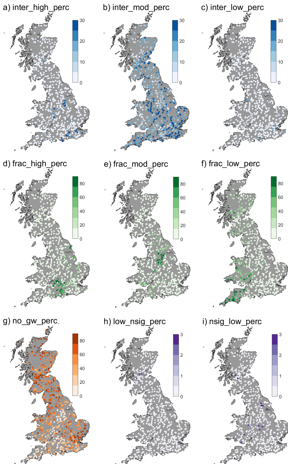
Figure S9. Maps of hydrogeology attributes across GB, a-c) significant intergranular flow – high,
