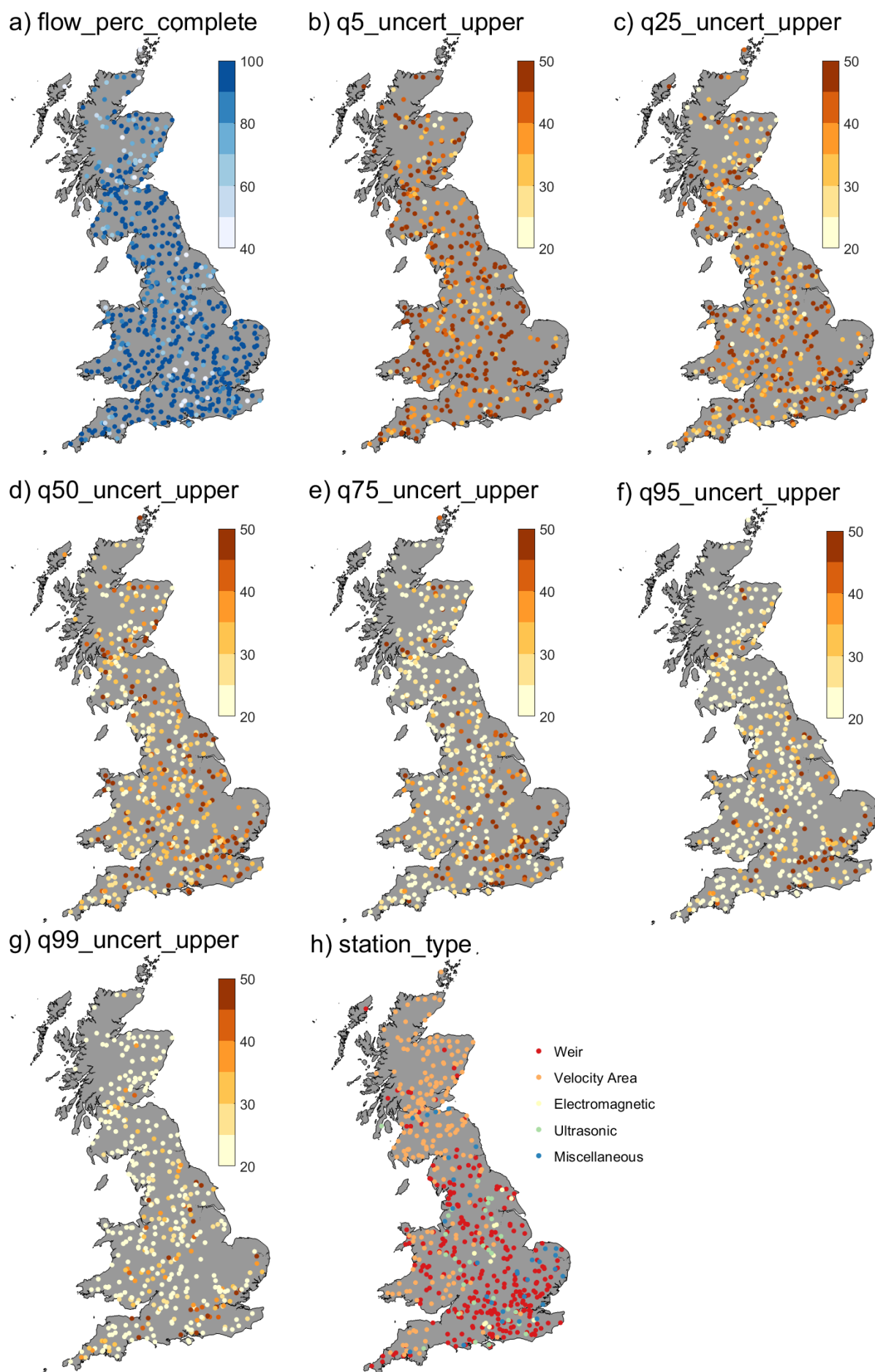
Figure S10. Maps of hydrometry attributes across GB, a) percentage of days with flow time series available from 1st October 1970 – 31st September 2015 (%), b-g) discharge uncertainty interval
