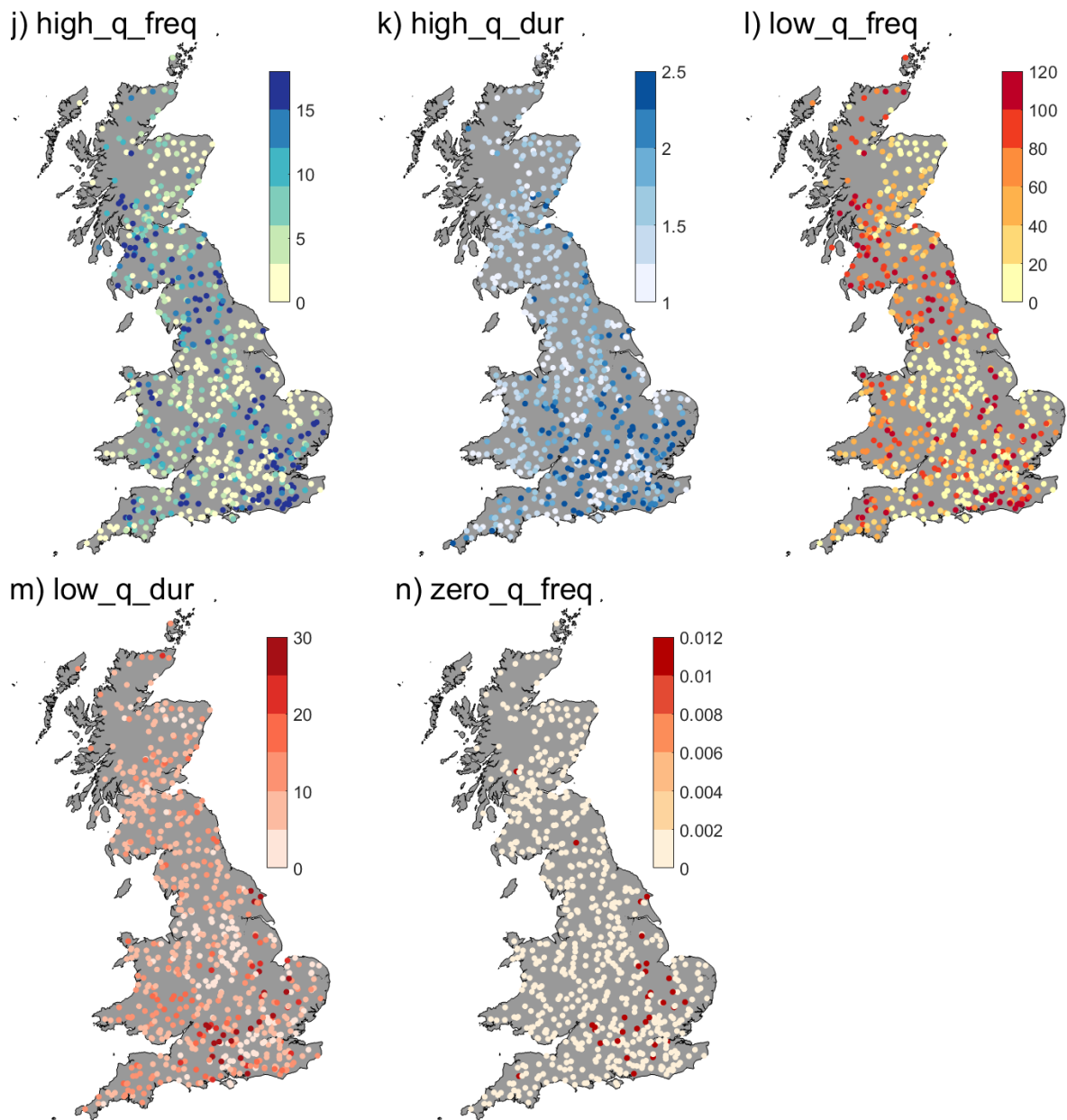
Figure S6. Maps of hydrologic signatures indices across GB, a) mean discharge (mm day -1 ), b) runoff ratio (-), c) stream elasticity (-), d) slope of the flow duration curve (-), e) base flow index (-), f) base flow index CEH (-), g) mean half flow date (day of year), h) Q5 (mm day -1 ), i) Q95 (mm day -1 ), j) frequency of high flow days (days yr -1 ), k) average duration of high flow events (days), l) frequency of low flow days (days yr -1 ), m) average duration of low flow events (days), n) frequency of days where flow equals zero
