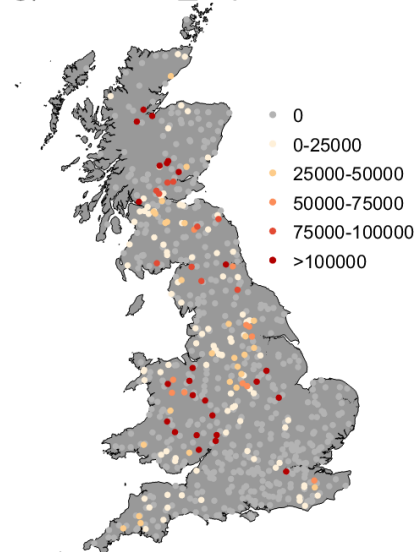
g) reservoir_cap
