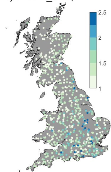
c) stream_elas
