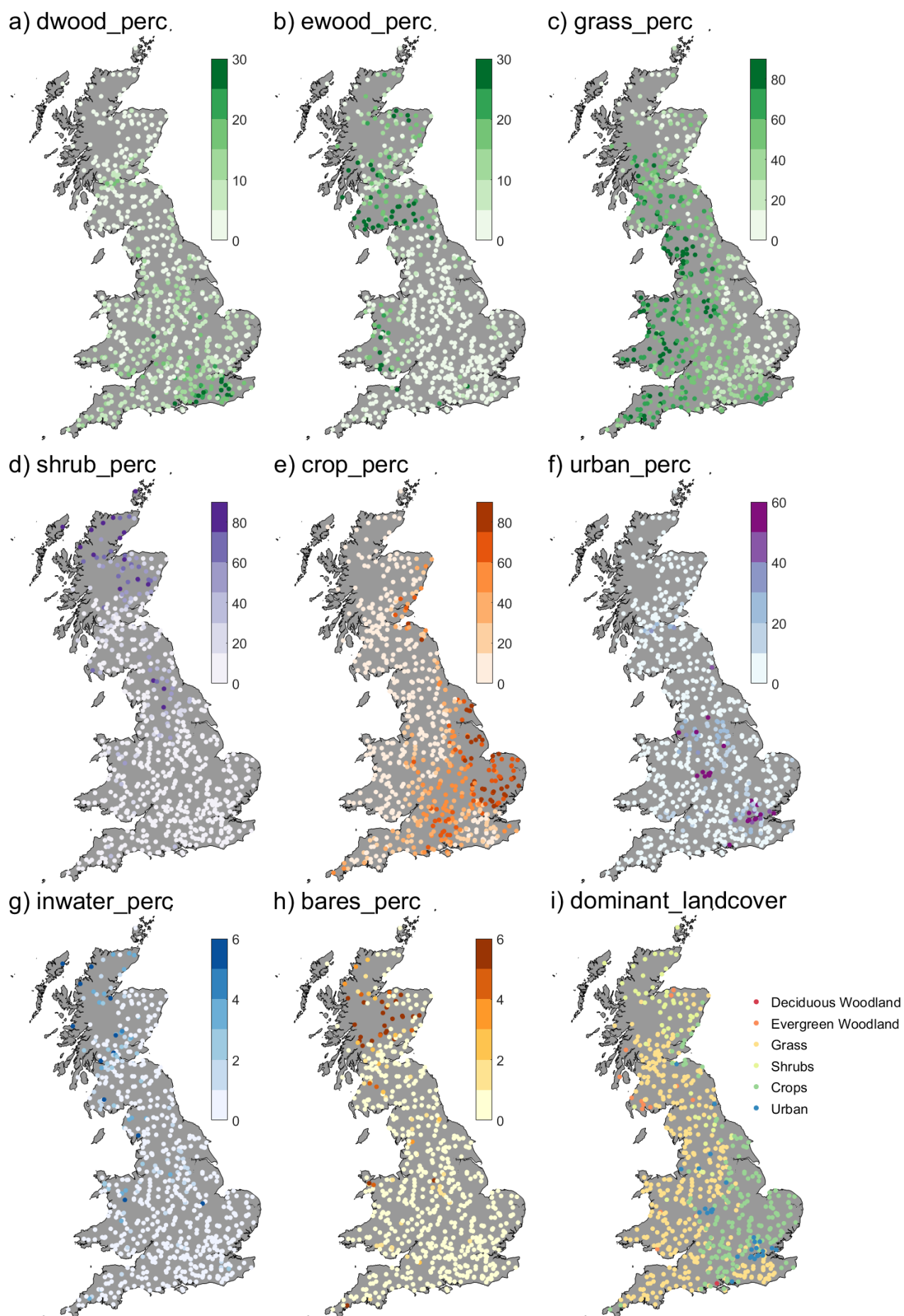
Figure S7. Maps of land cover attributes across GB, a) deciduous woodland (%), b) evergreen woodland (%), c) grass and pasture (%), d) shrubs (%), e) crops (%), f) urban and suburban (%), g) inland water (%), h) bare soil and rocks (%), i) dominant land cover (-)
