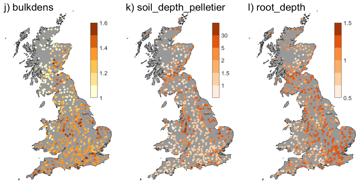
Figure S8. Maps of soil attributes across GB, a) percentage of clay (%), b) percentage of silt (%), c) percentage of sand (%), d) volumetric porosity – cosby (-), e) volumetric porosity – hypres (-), f) saturated hydraulic conductivity – cosby ( \text{cm h}^{-1} ), g) saturated hydraulic conductivity – hypres ( \text{cm h}^{-1} ), h) total available water content (mm), i) percentage of organic content (%), j) bulk density ( \text{g cm}^{-3} ), k) depth to weathered bedrock (m), l) depth available for roots (m)
