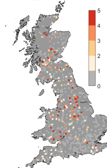
f) num_reservoir
