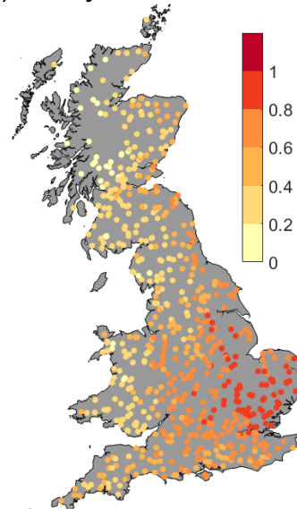
c) aridity
