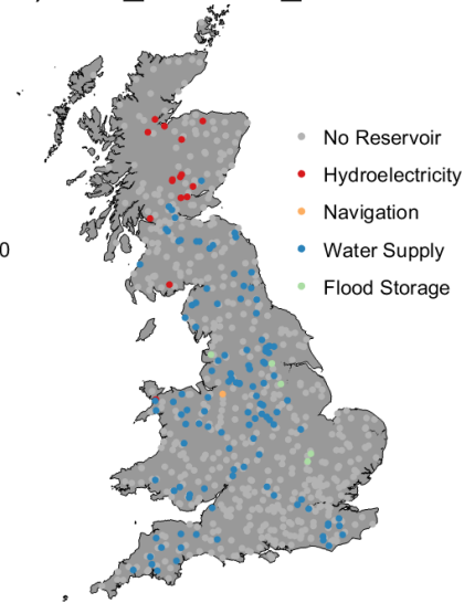
h) dom_reservoir_use
