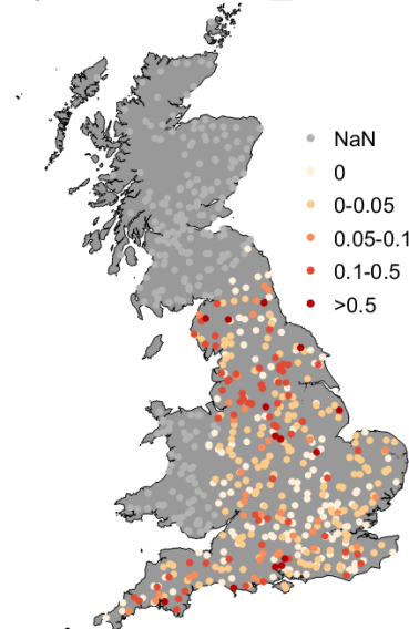
b) surfacewater_abs
