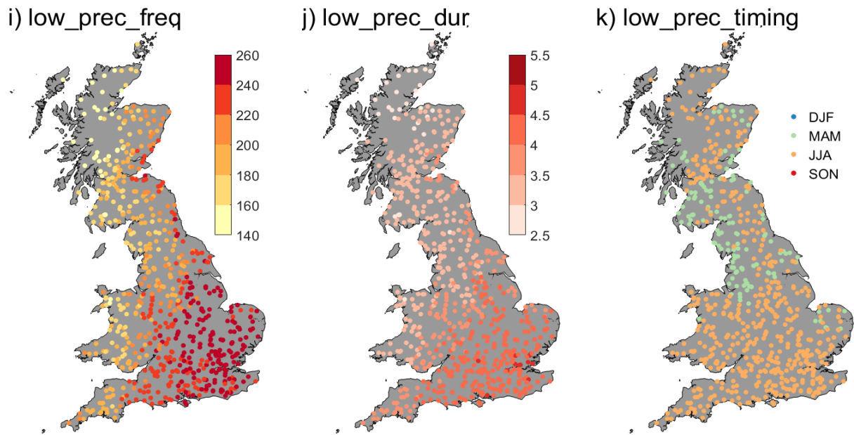
Figure S5. Maps of climatic indices across GB, a) mean precipitation (mm/day), b) mean potential evapotranspiration (mm/day), c) aridity (-), d) seasonality of precipitation (-), e) snow fraction (-), f) frequency of high precipitation days (days yr -1 ), g) average duration of high precipitation events (days), h) season during which most high precipitation days occur (season), i) frequency of dry days (days yr -1 ), j) average duration of dry periods (days), k) season during which most dry days occur (season)
