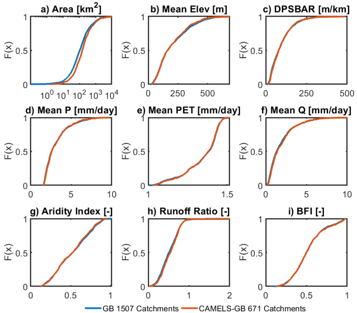
Figure S2. Cumulative distribution functions of key topographic, climatic and hydrologic catchment characteristics for all Great Britain catchments ( n=1507 ) and CAMELS-GB catchments ( n=671 ), a) catchment area ( \text{km}^2 ), b) mean catchment elevation (m), c) mean drainage path slope (m/km), d) mean precipitation (mm/day), e) mean potential evapotranspiration (mm/day), f) mean discharge (mm/day), g) aridity index (mean precipitation divided by mean potential evapotranspiration) (-), h) runoff ratio (mean discharge divided by mean precipitation) (-), i) base flow index (-)
