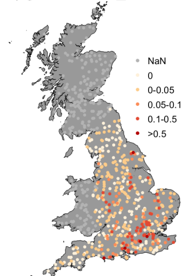
c) groundwater_abs
