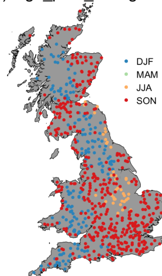
h) high_prec_timing
