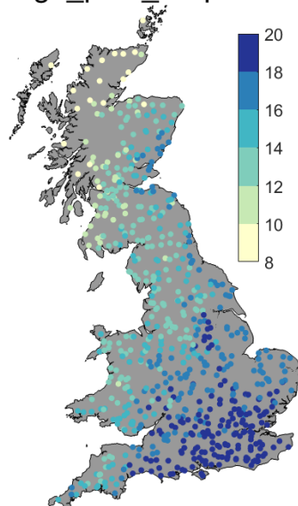
f) high_prec_freq
