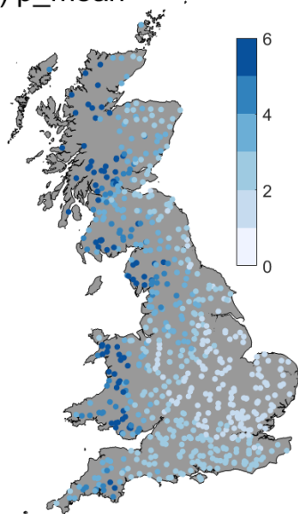
a) p_mean
