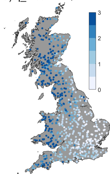
a) q_mean
