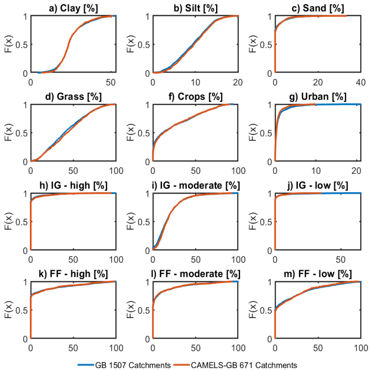
Figure S3. Cumulative distribution functions of key soil, land cover and hydrogeology catchment characteristics for all Great Britain catchments ( n=1507 ) and CAMELS-GB catchments ( n=671 ), a) percentage cover of clay (%), b) percentage cover of silt (%), c) percentage cover of sand (%), d) percentage land cover of grass (%), f) percentage land cover of crops (%), g) percentage cover of urban (%), h-j) significant intergranular flow – high, moderate and low productivity (%), k-m) flow predominantly through fractures – high, moderate and low productivity (%)
