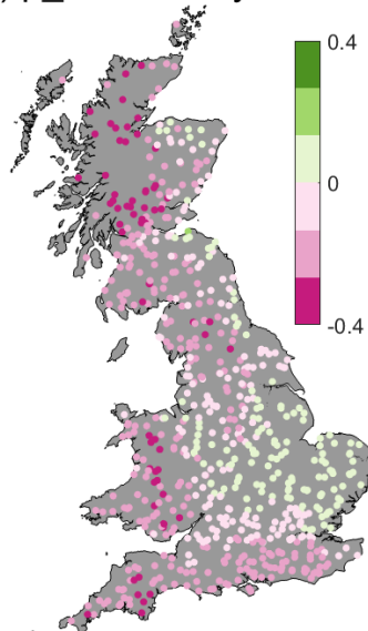
d) p_seasonality
