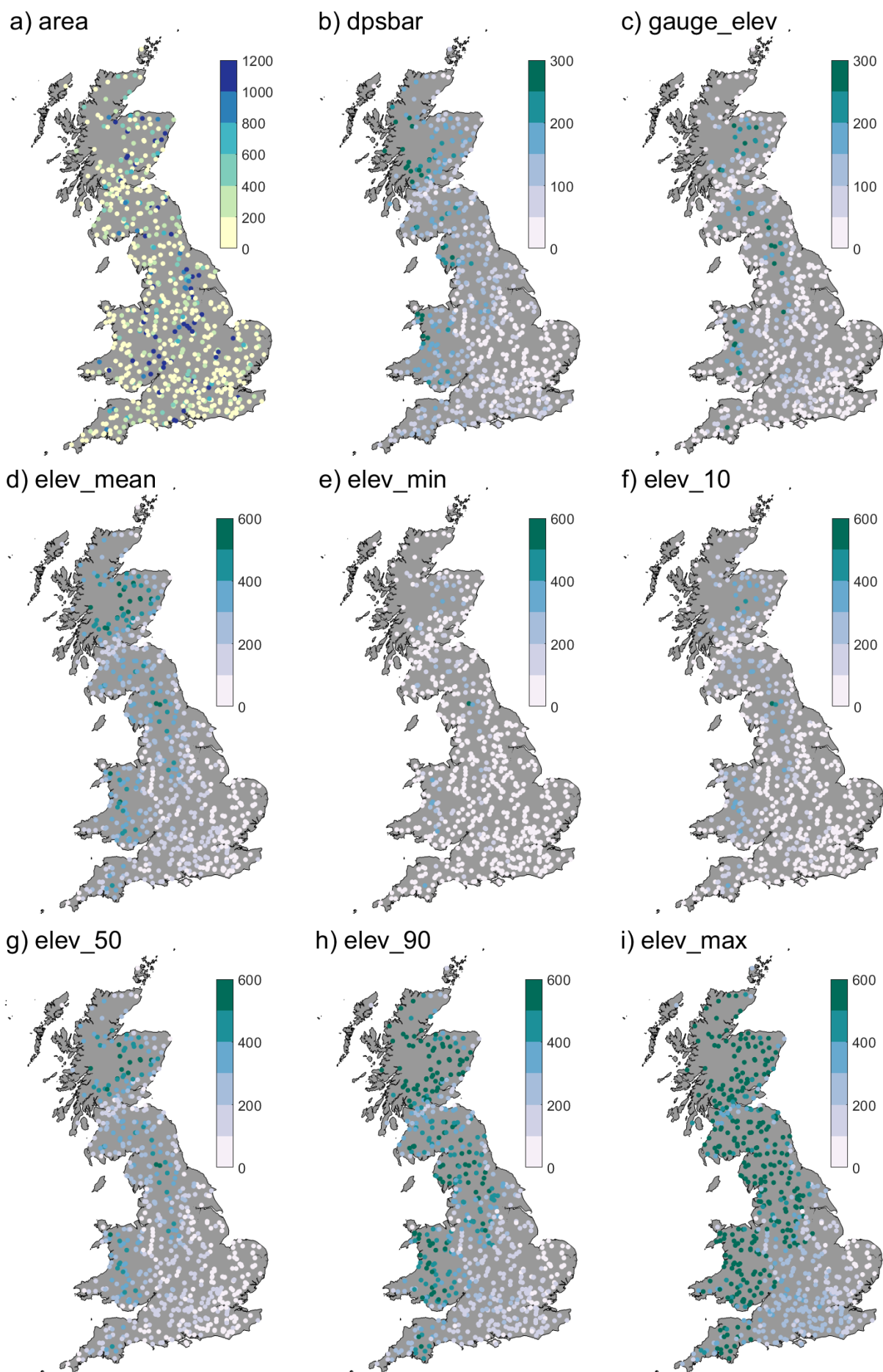
Figure S4. Maps of topographic attributes over GB, a) area (km 2 ), b) mean drainage path slope (m/km), c) gauge elevation (m), d) mean elevation (m), e) minimum elevation (m), f) 10 th percentile
