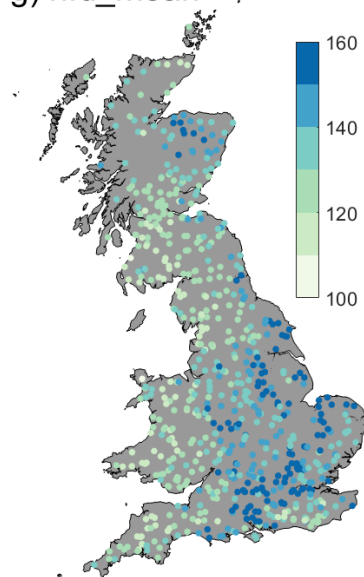
g) hfd_mean
