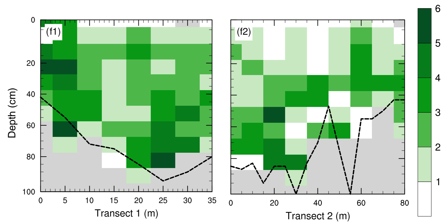
Nitrogen density ( \text{kg N m}^{-3} )
