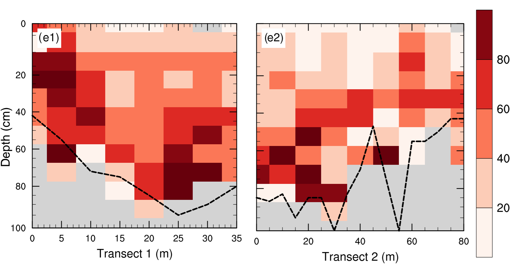
Carbon density ( \text{kg C m}^{-3} )
