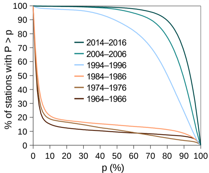
(a) P = \% \text{ Sfc-to-500 hPa hum. obs. (sfc. \& std. lev.)}
