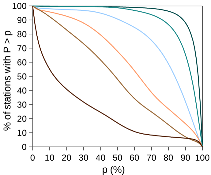
(b) P = \% \text{ Sfc-to-500 hPa hum. obs. (def. Sect. 2.3.4)}
