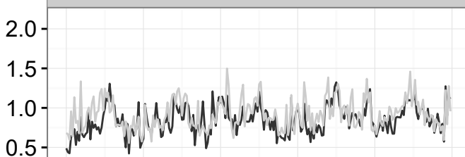
Sunshine duration
