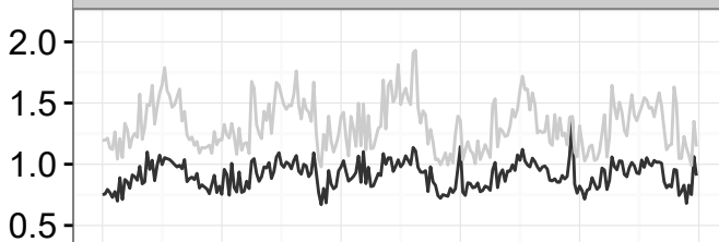
Maximum temperature
