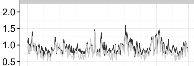
Wind speed
