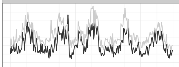
Dew point
