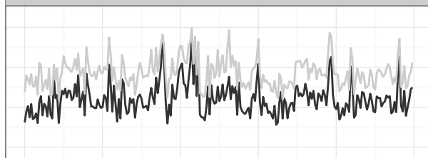
Minimum temperature
