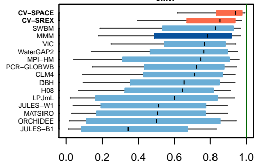
R^2_{clim}
