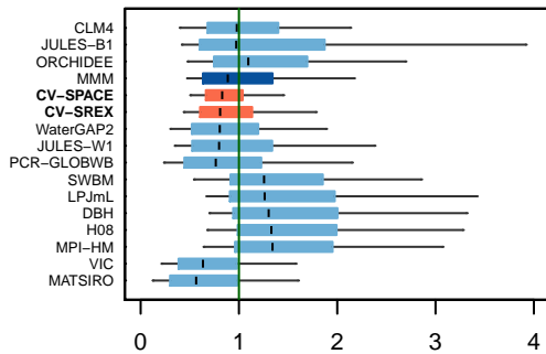
rSD
