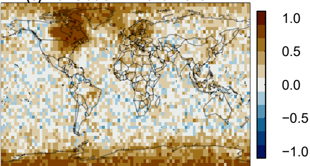
(c) Correlation: 12 040–7040 BP
