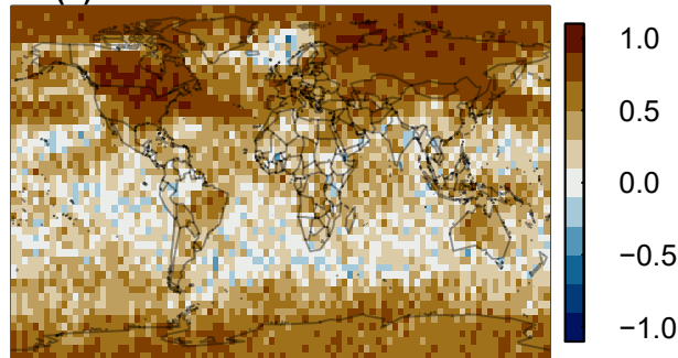
(b) Correlation: 17 040–12 040 BP
