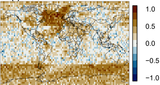
(a) Correlation: 22 040–17 040 BP
