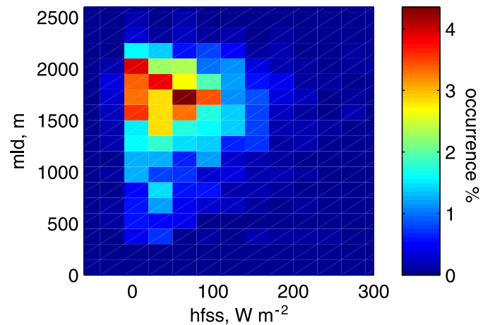
(a) mld/hfss occurrence JJA pm
