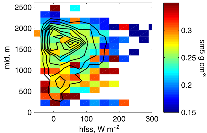
(c) 5 cm soil moisture JJA pm
