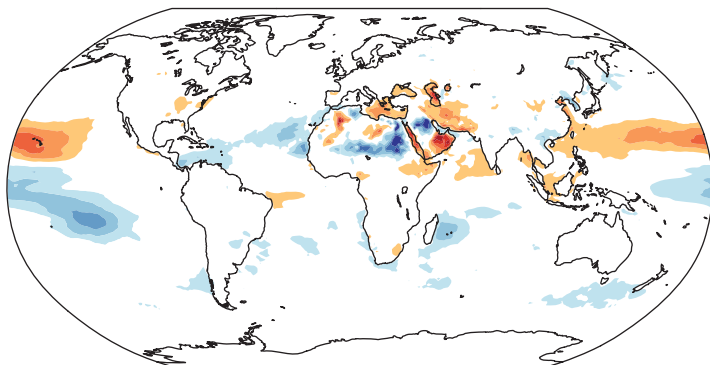
(b) Aerosol forcing (TOA)
