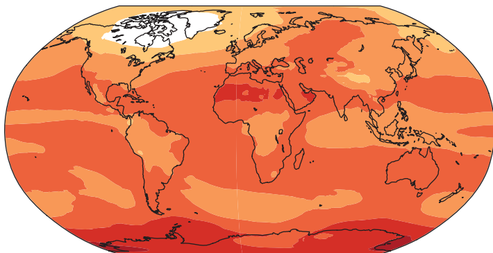
(a) Greenhouse gas forcing (TOA)
