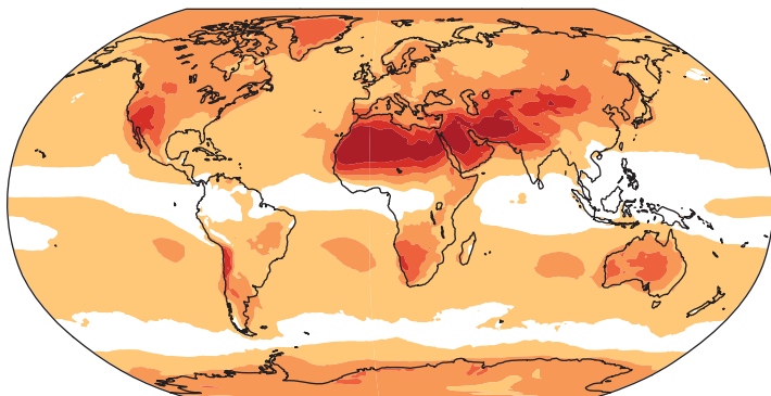
(c) Greenhouse gas forcing (surface)
