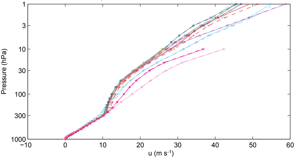
u averaged from 40 to 90° N on 1 Jan 1980 00:00 UTC
