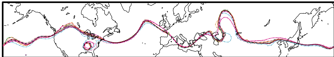
(c) Z = 5.5 km at 500 hPa
