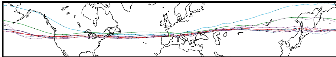
(b) Z = 30.5 km at 10 hPa
