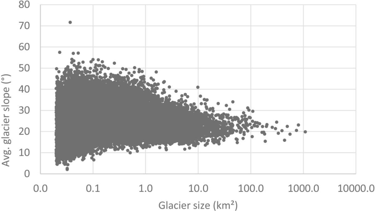
Fig. S1: Glacier slope vs. glacier size:
