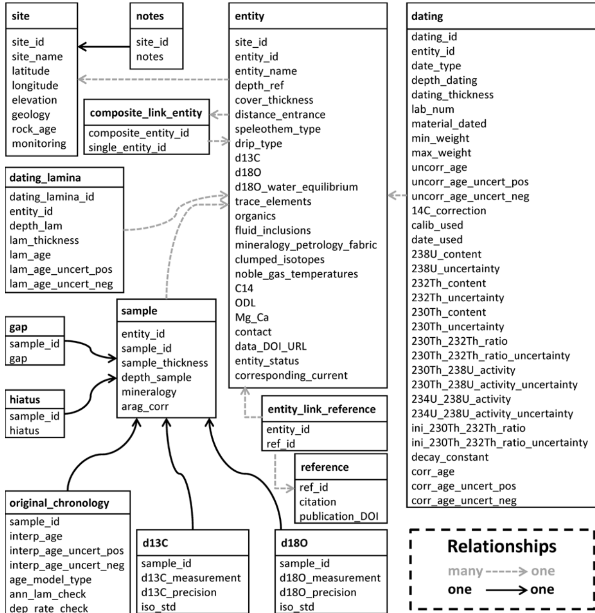
Figure S1: The structure of the SISAL database, showing individual tables (and their contents) and the nature of the relationships between them (where “many to one linkages” indicate that it is possible to have several entries in one table linked to a single entry in another table).
