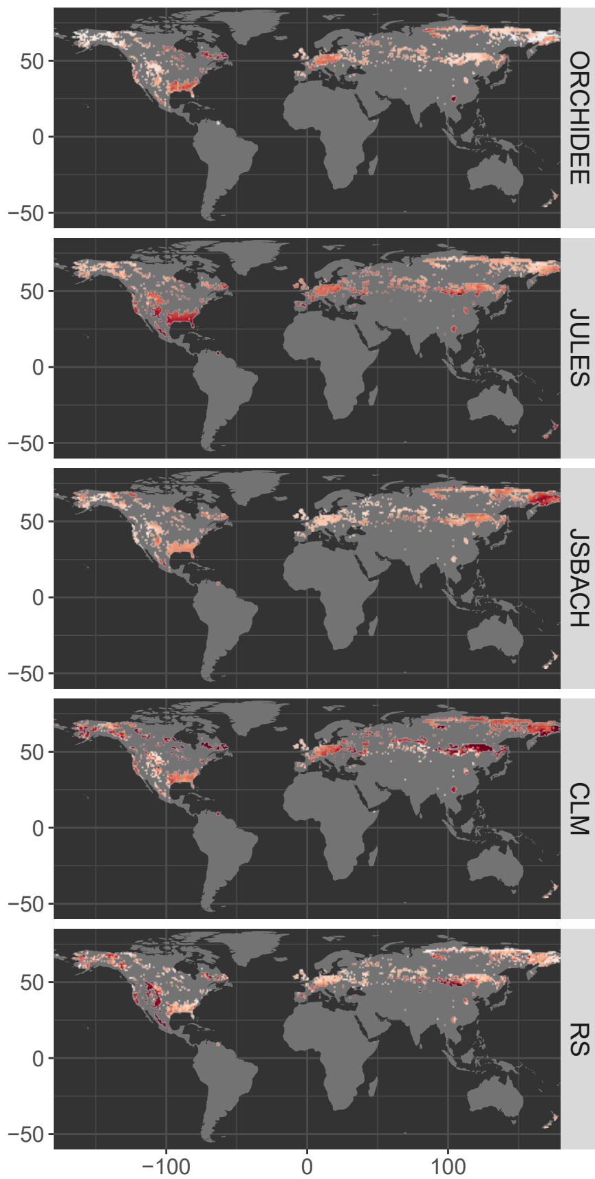
(a) Annual mean changes
