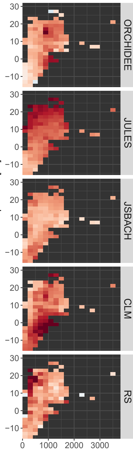
(c) Changes in climate space
