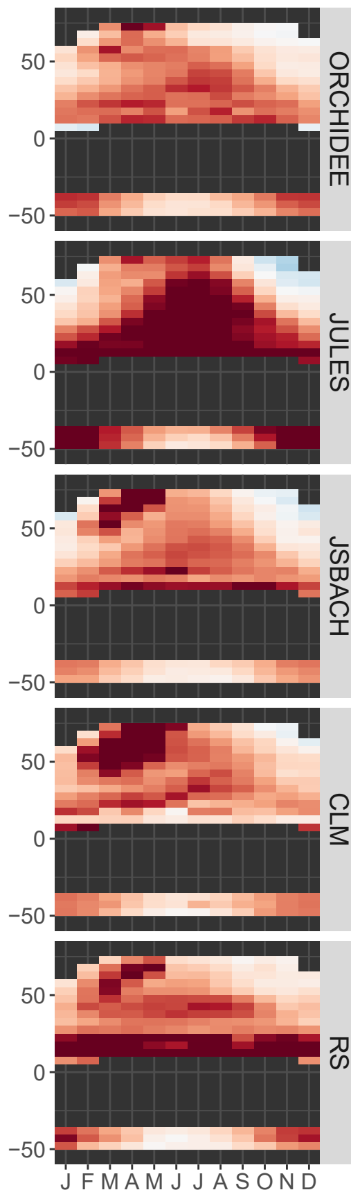
(b) Seasonal changes
